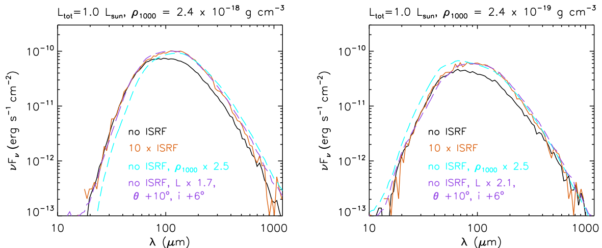
Figure 17. Similar to Figure 16, but for model SEDs with L_{tot}=1.0 L_{\odot} (black and orange lines). The light blue and purple dashed lines show SEDs from our model grid (no external heating) with the same model parameters as shown except for a reference density 2.5 times higher (light blue) and \theta=25^{\circ} , i=81^{\circ} , and a higher luminosity (purple).
