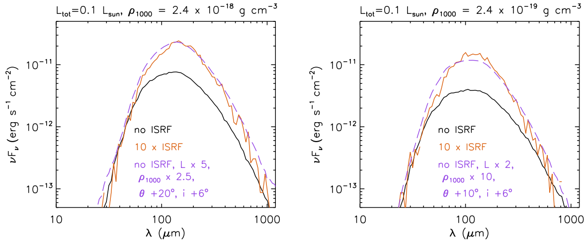
Figure 16. Black and orange lines: SEDs for models with L_{tot}=0.1 L_{\odot} , R_c=100 AU, \theta=15^{\circ} , i=75^{\circ} , reference densities \rho_{1000}=2.4 \times 10^{-18} g cm ^{-3} (left) and 2.4 \times 10^{-19} g cm ^{-3} (right), without external heating (black) and with heating by an ISRF scaled by a factor of 10 (orange). The purple dashed lines show SEDs from our model grid (which does not include external heating) with model parameters changed as indicated in the figure label; these models were chosen to closely match the model SEDs with external heating.
