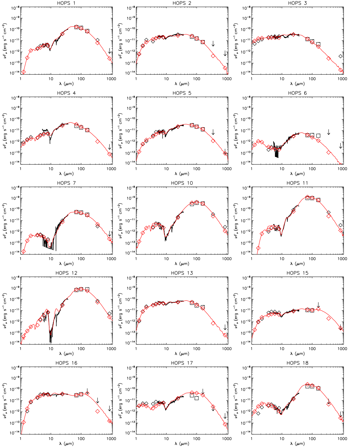
Figure AA1: SEDs of the HOPS targets modeled in this work ( black ; open symbols: photometry, arrows: upper limits, line: IRS spectrum). The best-fit model for each object is shown as a red line, with fluxes taken from a 4'' aperture for \lambda < 8 \mu\text{m} , a 5'' aperture for \lambda = 8 - 37 \mu\text{m} , and a 10'' aperture for \lambda > 37 \mu\text{m} . The red symbols are the model photometry measured in the same apertures and bandpasses as the data (see Section 4.2 for details).
