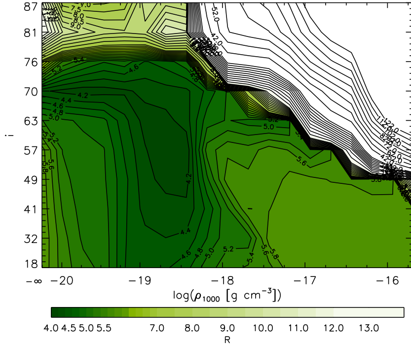
Figure CC2.: R contour plot for the models that fit HOPS 24. For each combination of inclination angle and reference density, the lowest R values of models with these two parameter values are shown. The remaining R contour plots are available in Figure Set C2.
