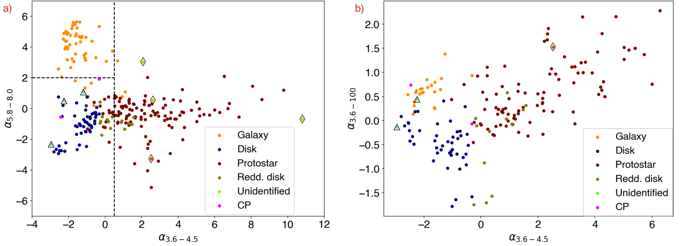
Figure 13. a) Plot showing \alpha_{5.8,8.0} vs. \alpha_{3.6,4.5} and b) \alpha_{3.6,100} vs. \alpha_{3.6,4.5} . Maroon diamonds and blue triangles denote reclassified protostars and pre-ms stars with disks, respectively. The horizontal and vertical dash lines in panel a denotes \alpha_{5.8,8.0} = 2 and \alpha_{3.6,4.5} = 0.5 , respectively
