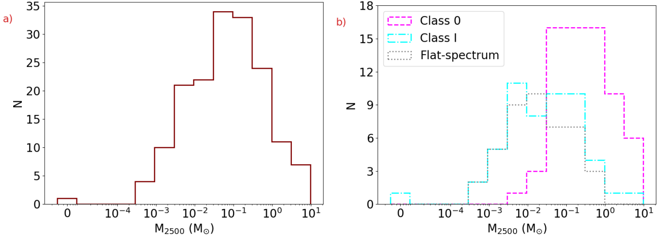
Figure 30. Panel a) Histogram of the model-derived envelope mass within 2500 au ( M_{2500} ) from the best fits of protostars in the eHOPS sample for Aquila. Panel b) Histogram of M_{2500} separated by different SED classes. Class 0 protostars have the highest M_{2500} . AD tests show significant differences in the distribution of M_{2500} between Class 0 and the remaining classes, but no significant difference between Class I and flat-spectrum sources.
