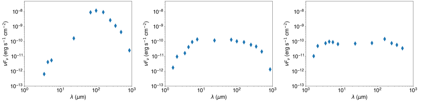
Figure 9. A few examples of SEDs of protostars in Aquila regions that are identified using Equation 7 defined in section 4.1.4. The sources are eHOPS-aql-67 (Class 0), eHOPS-aql-48 (Class I), and eHOPS-aql-2 (flat-spectrum), respectively from left to right. These protostars are identified as part of Step 3.
