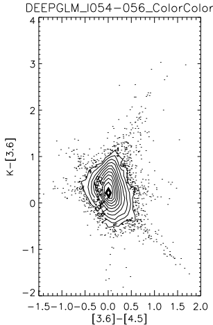
Figure 7: Color-color plot of the region l = 54^\circ - 56^\circ and b = +0.7^\circ to +2.8^\circ for sources in the Archive. 10 contours are evenly spaced between \log(\# \text{ sources/mag}^2) = 2.0 and the log of maximum number of sources per square magnitude. The contours are labeled with the log of the number of sources per square magnitude. Outside of the lowest contour, the positions of individual sources are plotted.
