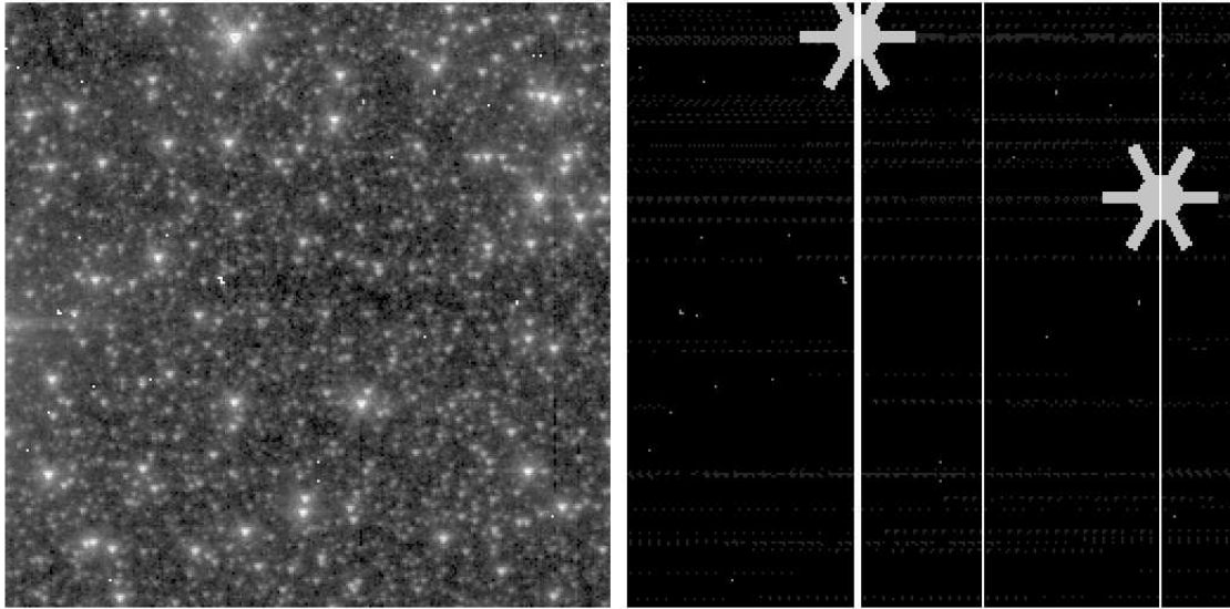
Figure 12: The IRAC [3.6] GLIMPSE frame (AOR 12110848, exposure 11) is on the left (corrections were applied for muxbleed and column pulldown); the flags for that frame are shown on the right. The PSF-shaped areas around the bright sources correspond to SQF bit 20. The vertical lines correspond to where the frame was corrected for column pulldown (SQF bit 15). The horizontal dots show which pixels were corrected for muxbleed (SQF bits 7 and/or 9). Various small dots are hot, dead or bad pixels (SQF bit 8). Bits in the SQF will have been set for sources within 3 pixels of any of these areas.
