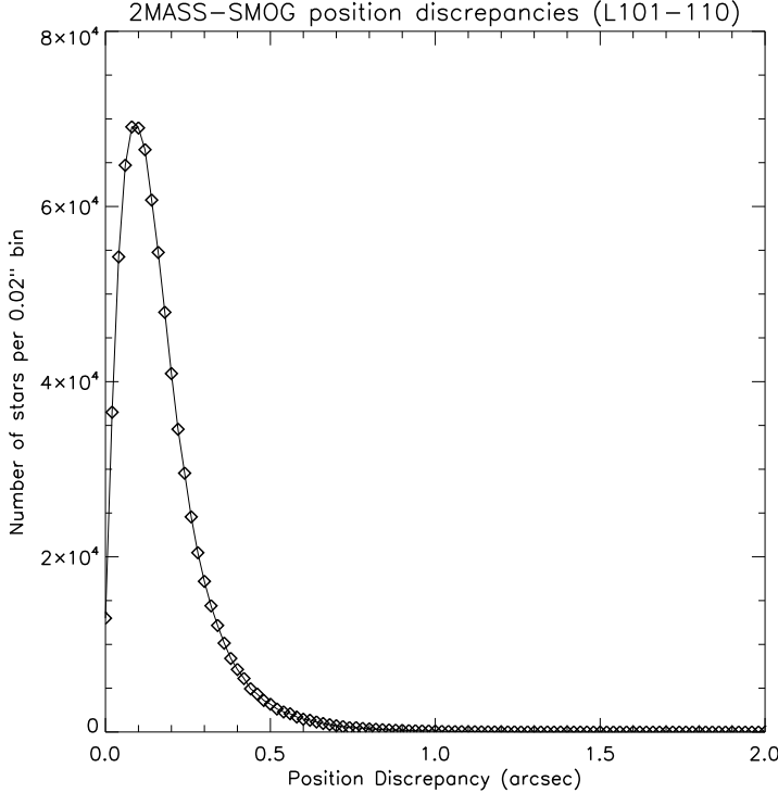
Figure 3: Comparison of SMOG source positions to their corresponding 2MASS PSC positions. The astrometric discrepancy plotted is the angular separation in arcseconds between the SMOG position and the 2MASS position. Note that sources with 2MASS associates have SMOG positions that are in part derived from the 2MASS position. Thus this is not a comparison of a pure IRAC-only position with the 2MASS position.
