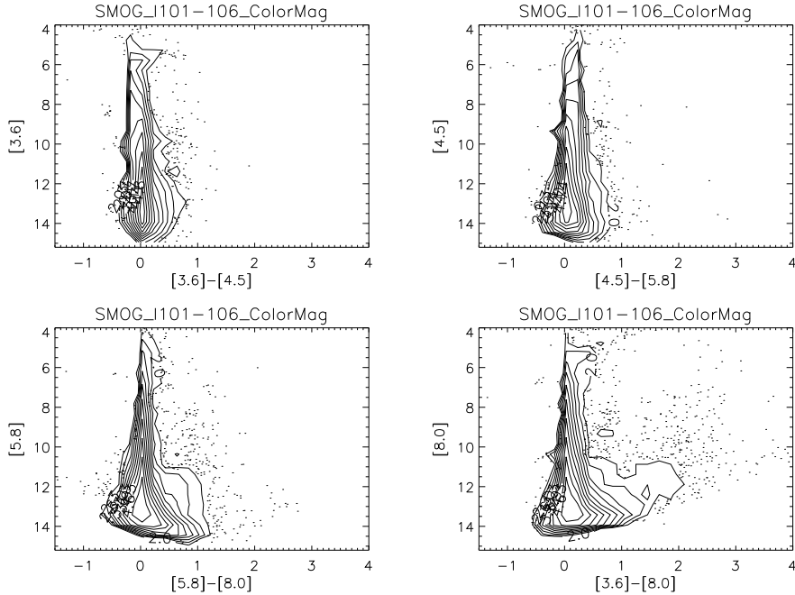
Figure 7: Same as Figure 7 except that these are Color-magnitude plots.
