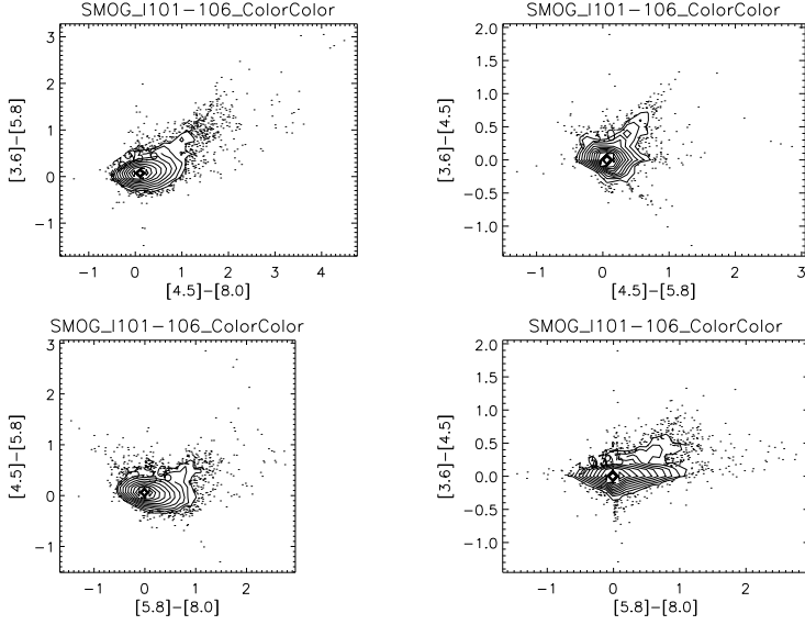
Figure 6: Color-color plot of the region l = 101^{\circ}-106^{\circ} for sources in the SMOG Archive. 10 contours are evenly spaced between \log(\# \text{ sources}/\text{mag}^2)=2.0 and the log of maximum number of sources per square magnitude. The contours are labeled with the log of the number of sources per square magnitude. Outside of the lowest contour, the positions of individual sources are plotted.
