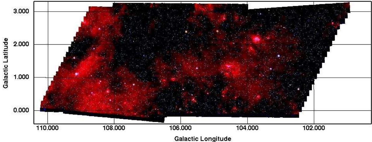
Figure 1: The area observed by the SMOG survey with the IRAC instrument. This is a 3-color image ([3.6], [4.5] and [8.0] in blue, green, and red respectively) of the survey region. IRAC source lists and enhanced images for the entire survey area have been delivered to IRSA.
