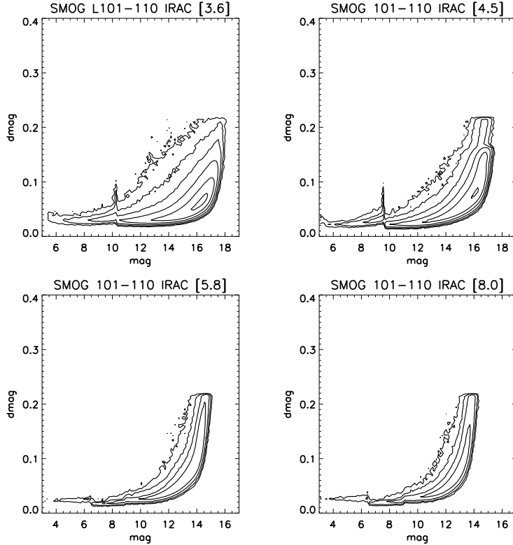
Figure 4: Magnitude uncertainty vs. magnitude for each IRAC band included in the SMOG Archive for the entire survey area. Contours show the density of sources. The lack of data above dmag of 0.22 is caused by the criterion that Archive data have signal to noise ratios of 5 or better. The “bump” at [3.6]=10.25 and [4.5]=9.6 is the boundary where the 0.6 sec framerate data are used for brighter sources and the 12 sec framerate data are used for fainter sources.
