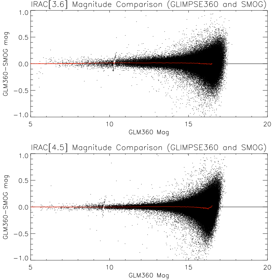
Figure 5: Comparison of GLIMPSE360 IRAC magnitudes with SMOG magnitudes at the l=109^\circ overlap region. Plotted in red is the mean difference (GLIMPSE360-SMOG) as a function of magnitude which is better than 0.02 mag for [3.6] and 0.01 for [4.5].
