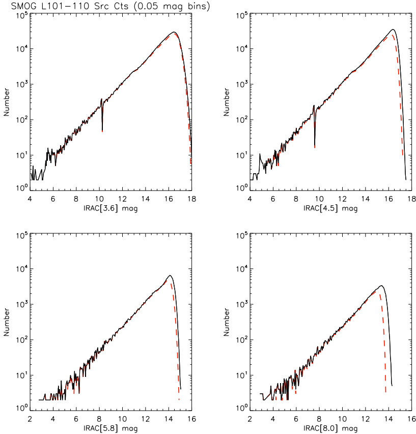
Figure 2: SMOG Catalog and Archive source counts versus magnitude for IRAC [3.6], [4.5], [5.8] & [8.0]. The dashed red lines are the Catalog; the black solid lines are the Archive. Included are all the SMOG data. The glitch in the [3.6] plot at 10.25 and the [4.5] plot at 9.6 are at the boundary where either the 0.6 sec FT data or the 12 sec FT data are used for photometry (see §3.3).
