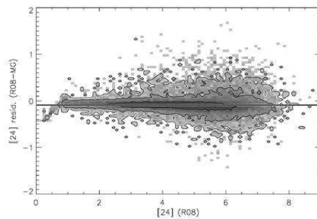
Fig. 6.— Photometry comparison of our MIPS-GAL archive to the MIPS-GAL photometry reported in Robitaille et al. (2008). Our calibration offset estimate is plotted as a solid line. The density map is inverted log scale, with white and black levels set to 1 and 10^3 sources per bin, respectively. Contours are plotted at 0.5, 5, and 50 sources per bin.
