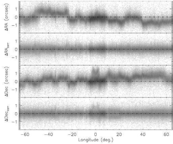
Fig. 2.— Astrometry residuals ( \Delta\text{RA} & \Delta\text{Dec}) to GLIMPSE positions versus Galactic Longitude before and after (“corr” subscript) correction of systematic astrometric offsets by tile, plotted as a source density map. The grayscale is inverted log scale, where white is <1 and black is >10^3 sources per bin. Residual spread in the “corr” plots is a combination of random variance and systematic variation within tiles that is partially correlated to MIPS scan legs.
