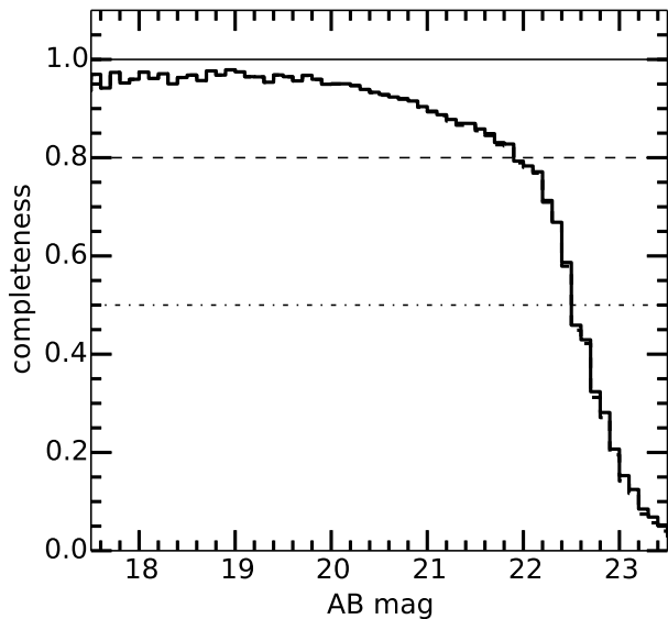
Figure 15. Completeness for point-sources in the SHELA data as a function of the input source magnitude. The plot shows the recovery fraction as a function of magnitude for simulated point sources, which are added to both the 3.6 and 4.5 \mu\text{m} images with the same AB magnitude. The solid-line histogram shows the raw completeness fraction. The dashed-line histogram shows the completeness corrected for “false positives” (sources that are “recovered” in the image, in which no simulated sources are added). The solid, dashed, and dot-dashed horizontal lines show 100%, 80%, and 50% completeness.
