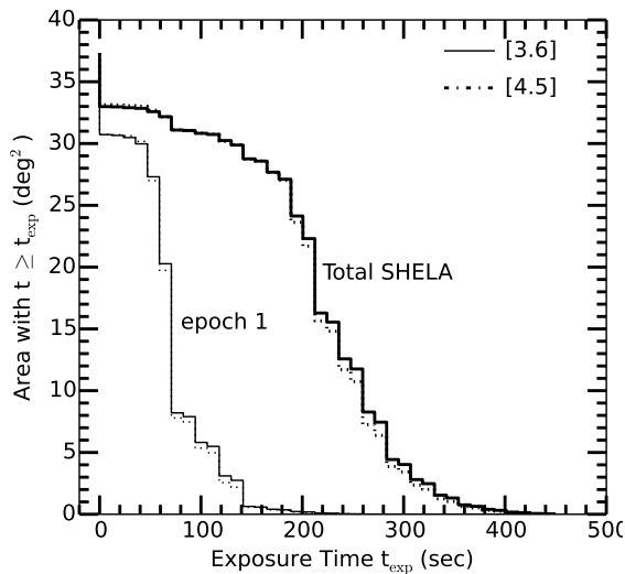
Figure 7. The cumulative distribution of area with exposure times \geq t_{\text{exp}} . The thin lines show the distribution only for the first epoch IRAC data, and the thick lines show the distribution for the combined three epoch data. The solid lines show the 3.6 \mu\text{m} distribution and the dotted line shows the 4.5 \mu\text{m} distribution.
