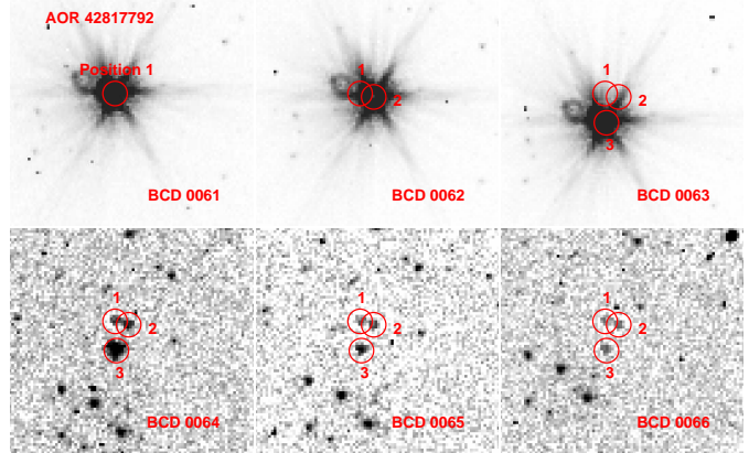
Figure 2. Example of persistence in the IRAC 3.6 \mu\text{m} data. The data are from AOR 42817792 of SHELA. Each panel shows the same region of the IRAC detector in a time series of sequential BCDs, from 0061–0066. In the first three BCDs (0061–0063), the bright star (HD 9670, V = 6.9 mag) falls at position 1, 2, and 3 in this portion of the IRAC detector. The bright star leaves a fractionally small persistence effect ( < 0.01\% of the fluence) in the same x,y pixels in subsequent BCDs (0064–0066), which decays with an exponential timescale.
