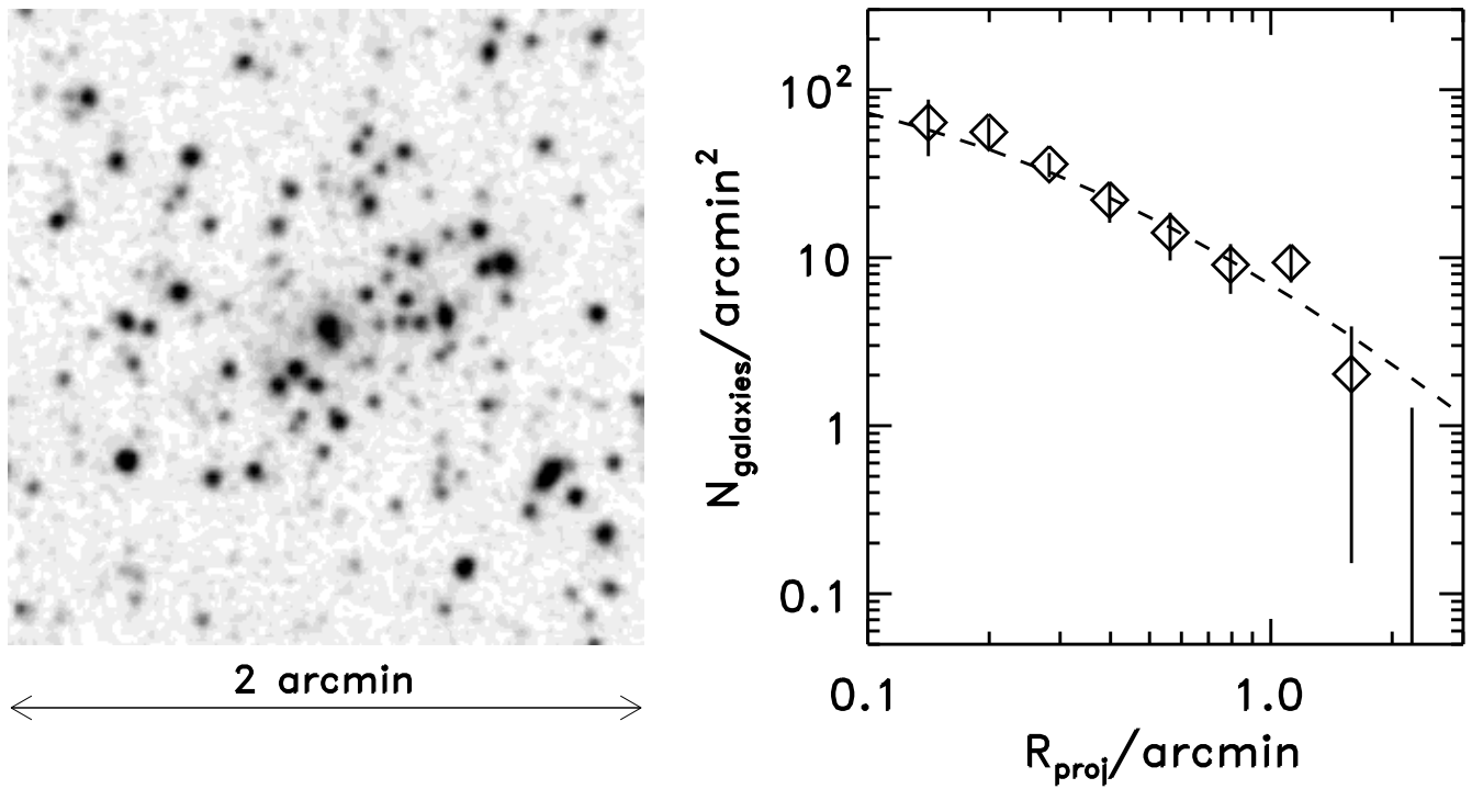
Figure 21. The left panel shows the SHEL A IRAC 3.6 \mu\text{m} image of the ACT SZ-selected cluster CLJ0058.0+0030 at z = 0.76 (Hasselfield et al. 2013). The right panel shows the projected surface-density distribution of galaxies centered on the peak of the SZ signal of the cluster. The surface density is the number of galaxies in the SHEL A IRAC data measured in concentric annuli centered on the cluster, corrected for the average density of galaxies in random apertures in the IRAC image. The surface density is consistent with a projected NFW profile with scale radius 0.51 \pm 0.14 arcmin.
