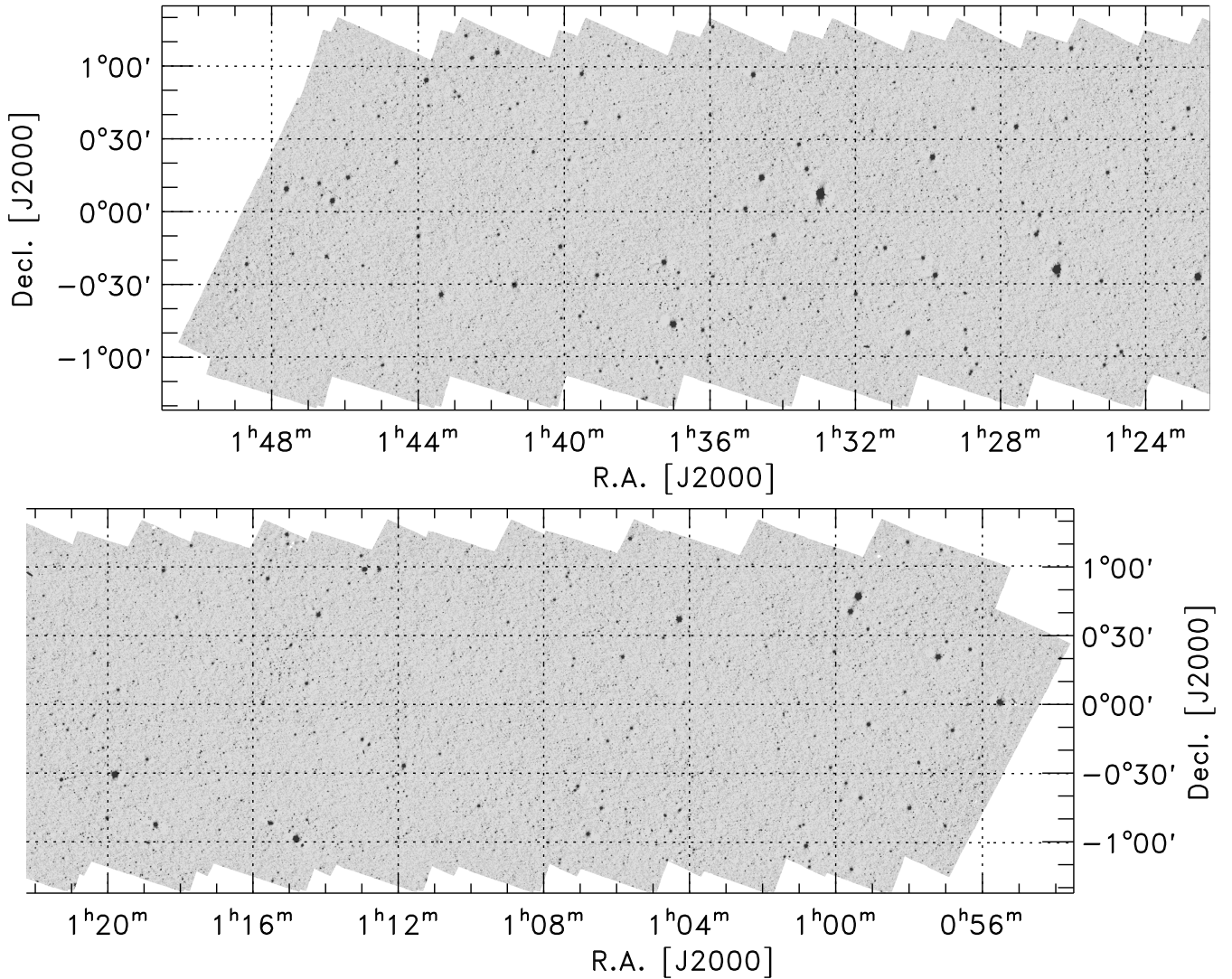
Figure 4. Same as Figure 3, but for the SHELA IRAC Channel 2 ( 4.5 \mu\text{m} ) data.
