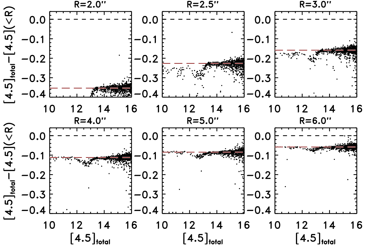
Figure 11. Same as Figure 10 for the SHELA IRAC 4.5 \mu\text{m} image.
