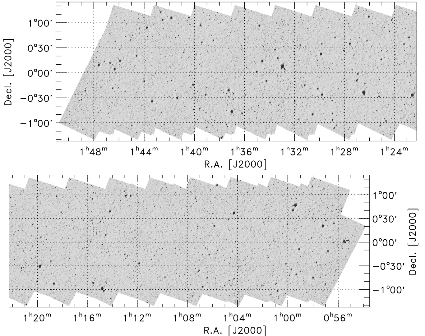
Figure 3. Combined, three-epoch mosaic of the SHELA IRAC Channel 1 ( 3.6 \mu\text{m} ) data. The extreme edges of the image cover nearly 2.5 \text{ deg} \times 13 \text{ deg} , but the area covered to our 3-epoch depth is \approx 24 \text{ deg}^2 .
