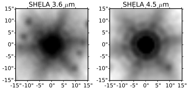
Figure 9. Empirical PRFs for the SHELA IRAC 3.6 and 4.5 \mu\text{m} data. The PRFs are constructed by combining the IRAC fluxes for point sources from the AllWISE catalog with magnitudes 14 < W1 < 15 Vega mag.
