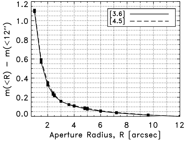
Figure 12. Aperture corrections for the IRAC images. The plot shows the difference between the IRAC photometric magnitude measured for point sources with magnitude between 13.5 and 16 mag in circular apertures of radius R and a total magnitude measured in an R = 12'' aperture. The aperture corrections are measured in apertures with discrete radii, as indicated by the solid black squares, and interpolated linearly between those points. The solid (dashed) line shows the 3.6 \mu\text{m} (4.5 \mu\text{m} ) data, as labeled in the plot legend.
