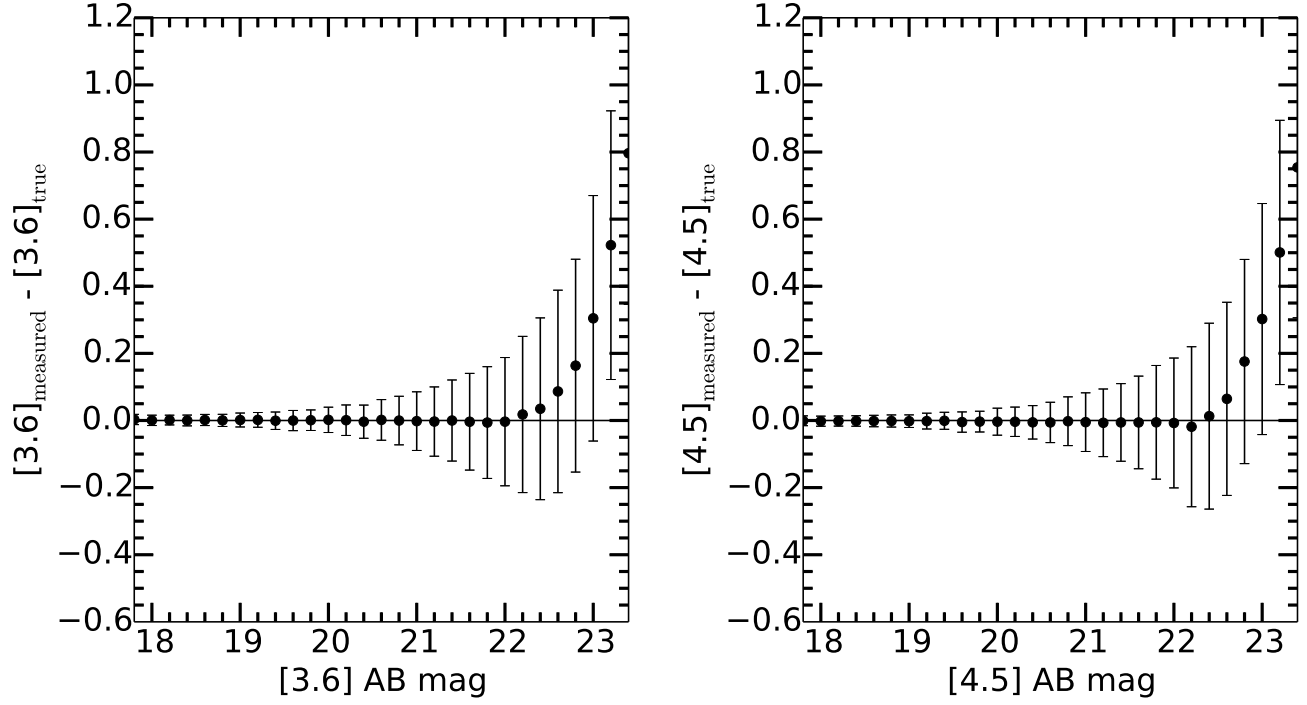
Figure 16. Comparison between the “true” (input) magnitude for simulated sources and the measured magnitude as a function of sources magnitude. The left panel shows the results for 3.6 \mu\text{m} , the right panel shows the results for 4.5 \mu\text{m} .
