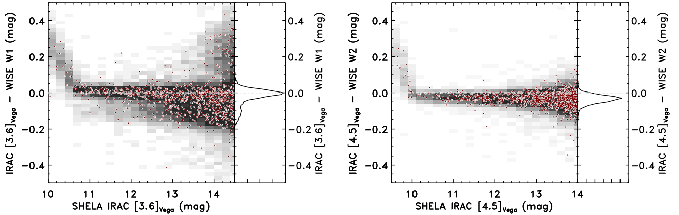
Figure 13. Comparison of magnitudes measured for point sources in the AllWISE catalog at 3.4 \mu\text{m} ( W1 ) and 4.6 \mu\text{m} ( W2 ) compared with those in the SHELA IRAC 3.6 and 4.5 \mu\text{m} data. Note that in this plot all magnitudes are relative to Vega-type stars. In both plots the gray shading shows all point sources, where darker regions correspond to a higher density of points falling in that region. The red points show a random subsample of the data. In each plot, the right panel shows the distribution of the magnitude difference between the IRAC and WISE image. The left plot compares the IRAC 3.6 \mu\text{m} and WISE W1 data. The photometric offset is negligible. The right plot compares the IRAC 4.5 \mu\text{m} and WISE W2 data. There is a small offset, -0.028 \text{ mag} . Stars brighter than \lesssim 10 ( 11 ) Vega mag appear saturated in the IRAC 3.6 ( 4.5 ) \mu\text{m} data.
