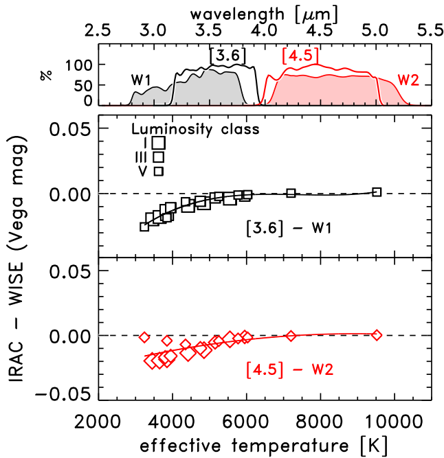
Figure 14. Expected differences between the IRAC and WISE photometry due to color variations in stars of different spectral type. The top panel compares the transmittance of the IRAC [3.6] and [4.5] filters to the WISE W1 and W2 filters. The plot shows synthesized colors between IRAC 3.6 \mu\text{m} and WISE W1 , and between IRAC 4.5 \mu\text{m} and WISE W2 . The data points correspond to Kurucz (1993) models for dwarfs (luminosity class V), giants (class III), and supergiants (class I) over a range of effective temperature (spectral type). Because the WISE instrumental filters are wider, they can include bandhead absorption features in late-type stars, affecting the IRAC–WISE color up to 0.03 \text{ mag} .
