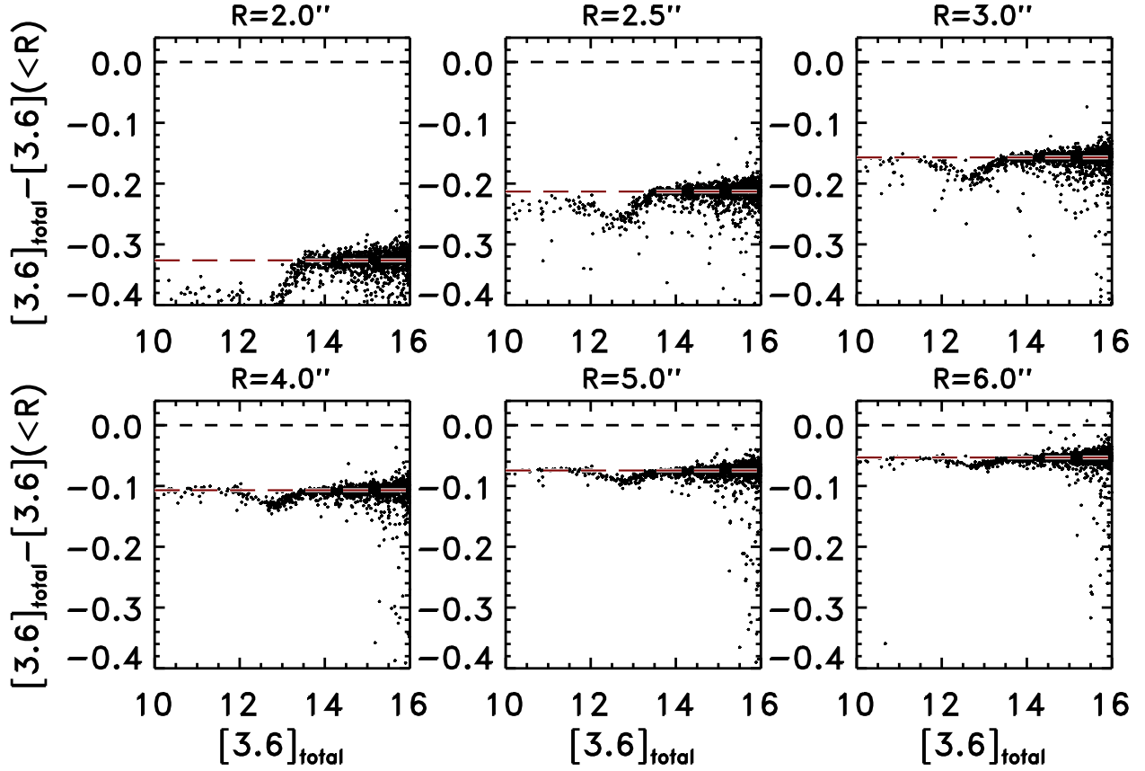
Figure 10. Estimate of light lost outside circular apertures of varying radius in the SHELA IRAC 3.6 \mu\text{m} image. Each panel shows the difference between a total magnitude (defined in a 12'' -radius aperture) and the magnitude measured in a smaller circular aperture of radius R for point sources from the AllWISE catalog. Each panel shows a different aperture radius R , given above each panel. The dashed, thick red line in each panel shows the median difference for stars between 13.5 < [3.6] < 16 mag, used to derive the aperture correction.
