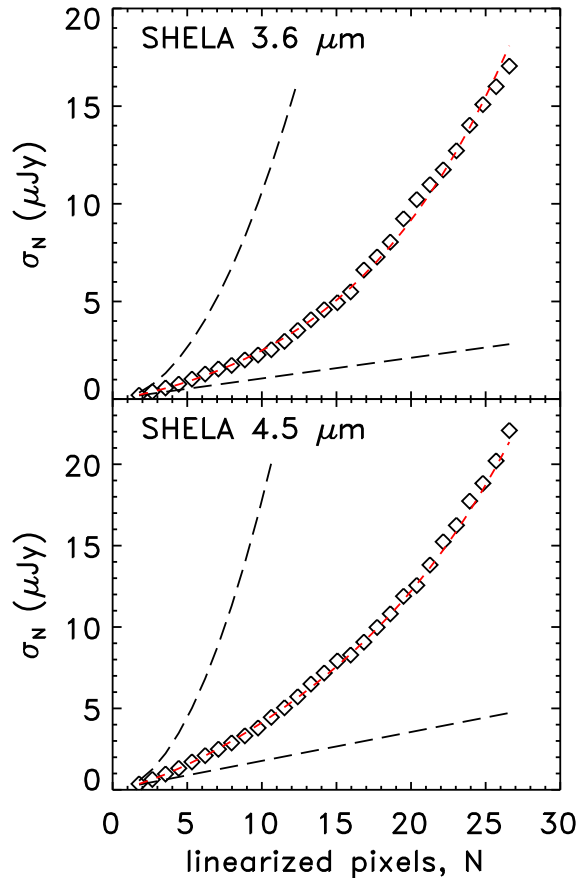
Figure 18. Scaling relation between the measured noise in the SHELA IRAC images and the number of linearized pixels, N = \sqrt{A} (where A is the area of the photometric aperture). Both panels show the measured noise, \sigma_N , in each aperture N . The top panel shows the 3.6 \mu\text{m} data and the bottom panel shows the 4.5 \mu\text{m} data. In each panel, the bottom-most dashed line shows the theoretical relation assuming uncorrelated pixels in the Gaussian limit, \sigma_N \sim N . The top-most dashed line shows the relation for perfectly correlated pixels ( \sigma_N \sim N^2 , Quadri et al. 2007). The red, short-dashed line shows the parameterized fit to the data, which we use to define the flux uncertainties measured in different-sized apertures.
