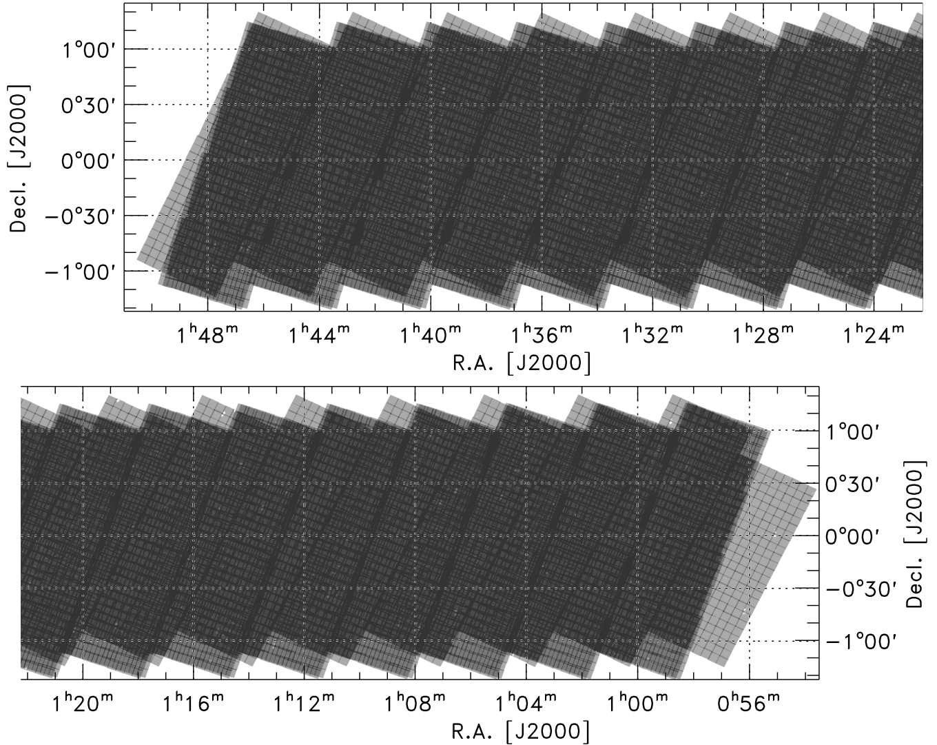
Figure 6. Same as Figure 5, for the SHELA IRAC Channel 2 ( 4.5 \mu\text{m} ) data.
