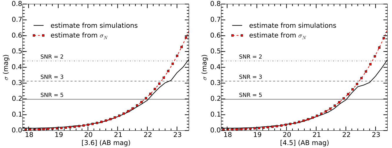
Figure 17. Estimates of uncertainties for the SHELA IRAC data. The left panel shows the results for the IRAC 3.6 \mu\text{m} data. The right panel shows the results for the 4.5 \mu\text{m} data. In each panel, the solid-line curve shows the estimated uncertainty measured from a comparison of the recovered magnitudes to the input magnitudes for fake sources added to the images. The points connected by the dashed-line curve show the estimates derived from \sigma_N for 2'' -radii apertures, scaled to total magnitudes. The horizontal lines show the equivalent magnitude uncertainty for a source with \text{SNR}=5, 3 , and 2 , as labeled.
