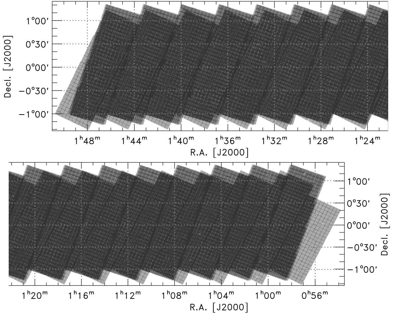
Figure 5. Combined, three-epoch exposure-time map of the SHELA IRAC Channel 1 ( 3.6 \mu\text{m} ) data.
