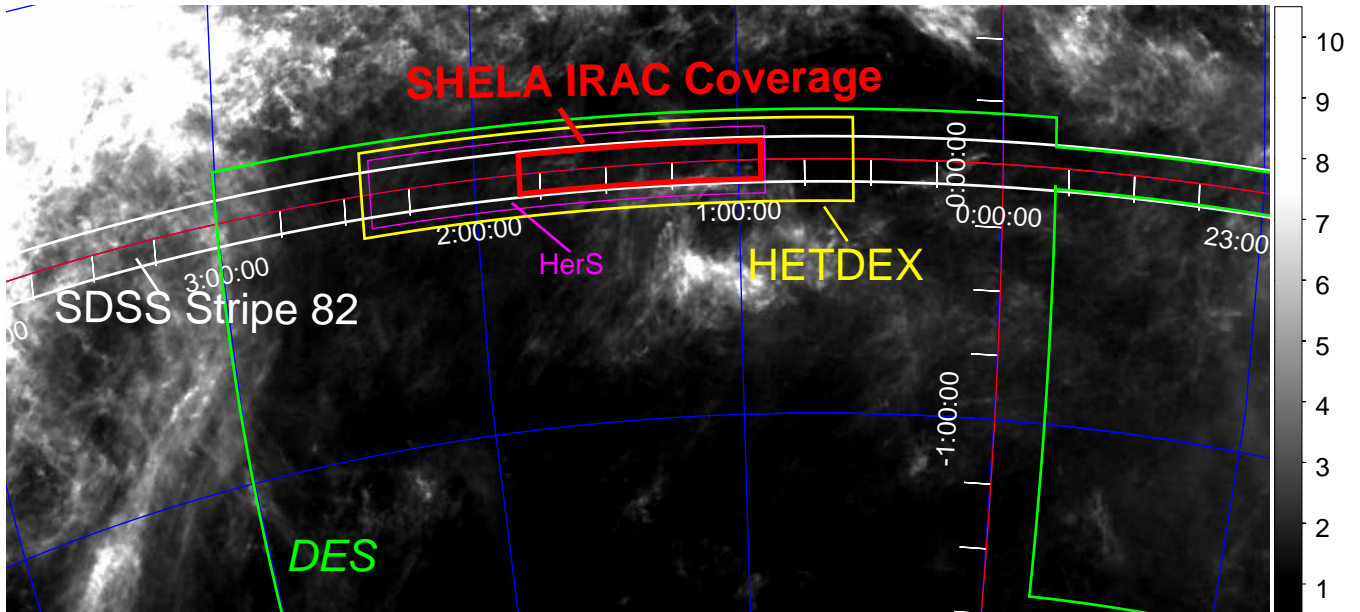
Figure 1. Field layout for SHELA. The thick lines show the coverage of our SHELA IRAC data (thick red-lined region), the SDSS Stripe 82 coverage (white-lined region), the planned coverage of the full-field of the HETDEX survey (yellow-lined region), the HerS Herschel coverage (magenta-lined region) and the planned coverage of the DES (green-lined region). The lines of constant R.A. and Decl. are labeled. The background image shows the IRAS 100 \mu\text{m} map of a portion of the south Galactic Pole (Schlegel et al. 1998). The image intensity scales with surface brightness as indicated in the color bar in units of MJy/sr.
