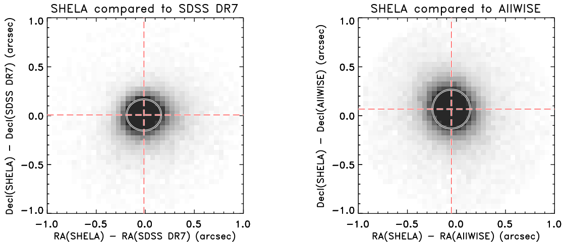
Figure 8. Astrometric comparison for point sources between the SHELA/IRAC and SDSS DR7 (left panel) and between SHELA/IRAC and AllWISE (right panel). In each panel, the shading is proportional to the density of objects in each region of the plot. The red, dashed lines show the mean offset. The ellipses contain 68% of the sources. There are negligible offsets between SDSS DR7 and SHELA (by construction), and the scatter is consistent with the SDSS astrometric accuracy of 0''.2 (Abazajian et al. 2009). In contrast, the AllWISE astronomy has a non-negligible offset of \approx 60 – 70 mas in both R.A. and Decl., with a scatter of 0.2'' in each dimension.
