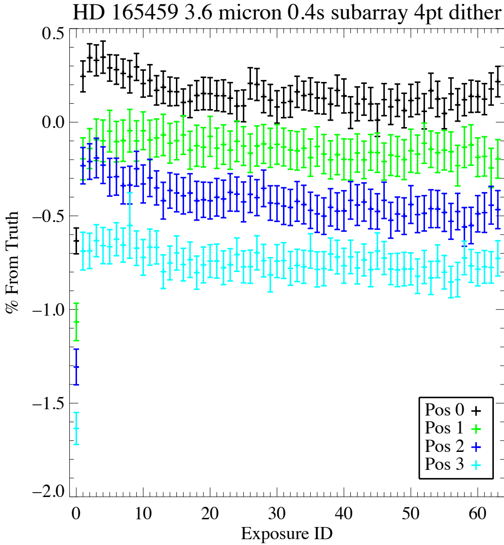
Figure 3: Variation of measured photometry compared to truth estimate as a function of subframe in each BCD and dither position.
