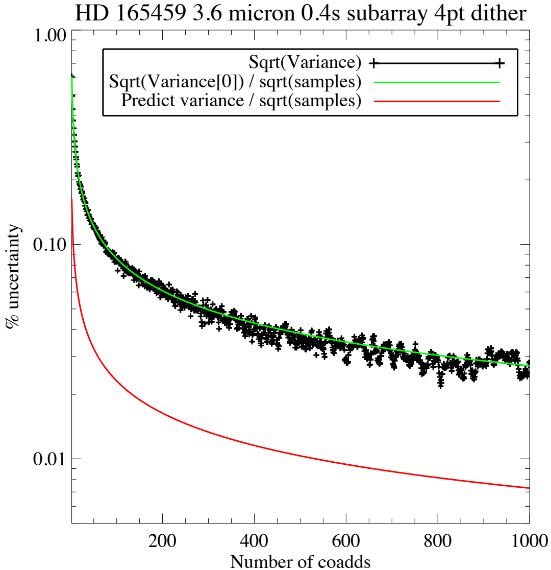
Figure 2: Variation in uncertainty as a function of averaging. The green curve is the N^{-0.5} trend scaled to the first data point. The red line is the expected uncertainty estimated from the readnoise and photon noise contributions.
