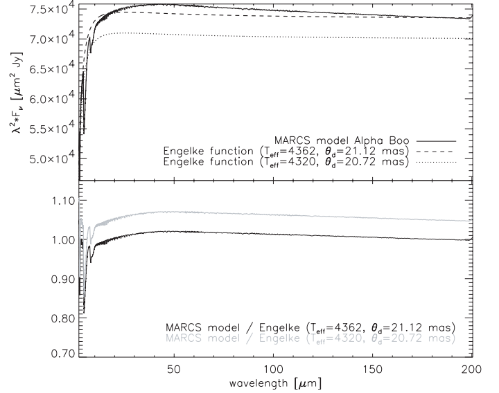
Fig. 11. Upper panel: comparison between the MARCS model spectrum of \alpha Boo ( \lambda/\Delta\lambda = 100 ) and predictions using the Engelke function with parameters T_{\text{eff}} = 4362 K and \theta_d = 21.12 mas (dashed line), and T_{\text{eff}} = 4320 K and \theta_d = 20.72 mas (dotted line). Bottom panel: ratio between MARCS model predictions and both Engelke functions.
