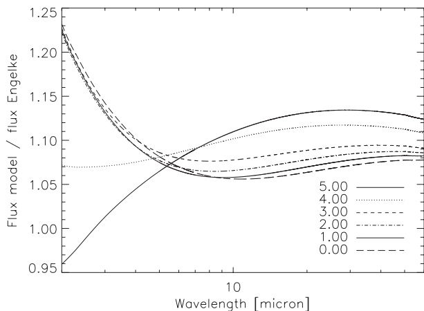
Fig. 1. Ratio between the continuum flux predicted from a theoretical plane-parallel stellar atmosphere with T_{\text{eff}} = 3500 K and values for the logarithm of the gravity ranging between 5.00 and 0.00 and the flux computed from the Engelke function.
