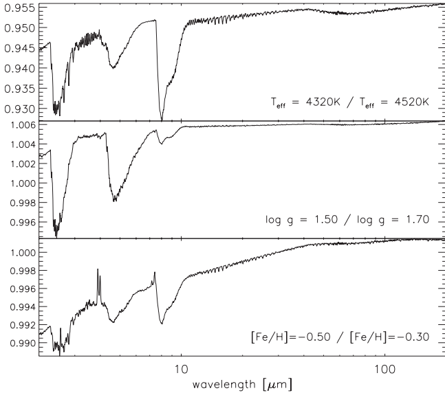
Fig. 8. Ratio between synthetic spectra with differing stellar parameters at a resolution of \lambda/\Delta\lambda = 100 . The standard model has the same stellar parameters as in Fig. 7. Upper panel: ratio between a synthetic spectrum with T_{\text{eff}} = 4320 K and with T_{\text{eff}} = 4520 K. Middle panel: ratio between \log g = 1.50 and \log g = 1.70 . Bottom panel: ratio between [\text{Fe}/\text{H}] = -0.50 and [\text{Fe}/\text{H}] = -0.30 .
