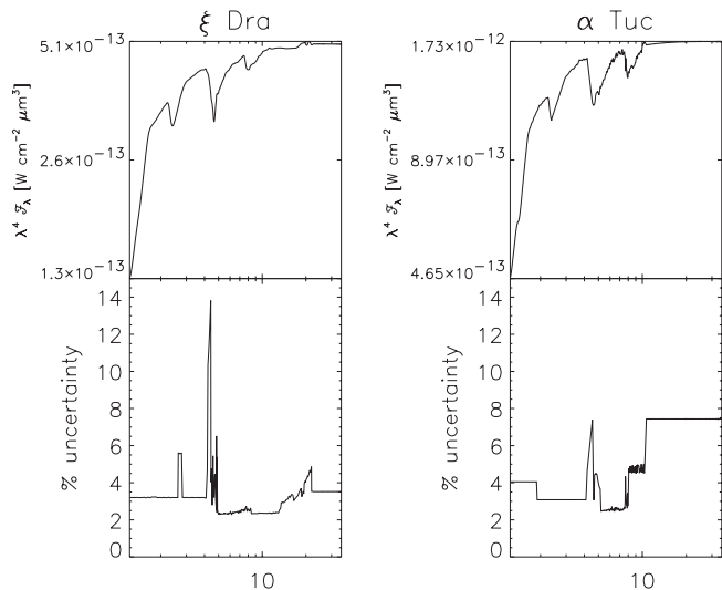
Fig. 5. Upper panels: Template spectra of \xi Dra (K2 III) and \alpha Tuc (K3 III). The composite spectrum of \alpha Boo (K2 IIIp) has been used to construct the template of \xi Dra (K2 III), and for \alpha Tuc (K3 III) the composite of \alpha Hya (K2 II-III) is used. Lower panels: the total uncertainty attributed to the templated spectra by Cohen et al. (1999). Main absorption features are the CO fundamental around 4.5 \mu\text{m} , CO first overtone around 2.3 \mu\text{m} , SiO fundamental around 8 \mu\text{m} and SiO first overtone around 4.2 \mu\text{m} .
