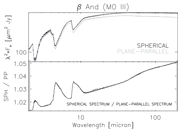
Fig. 2. Upper panel: model atmosphere spectrum in spherical geometry (black) compared to the theoretical spectrum calculated in plane-parallel geometry (grey) representing the M0 III giant \beta And ( \lambda/\Delta\lambda = 100 ). Bottom panel: ratio between spherical and plane-parallel spectrum. Stellar parameters are taken from Decin et al. (2003a).
