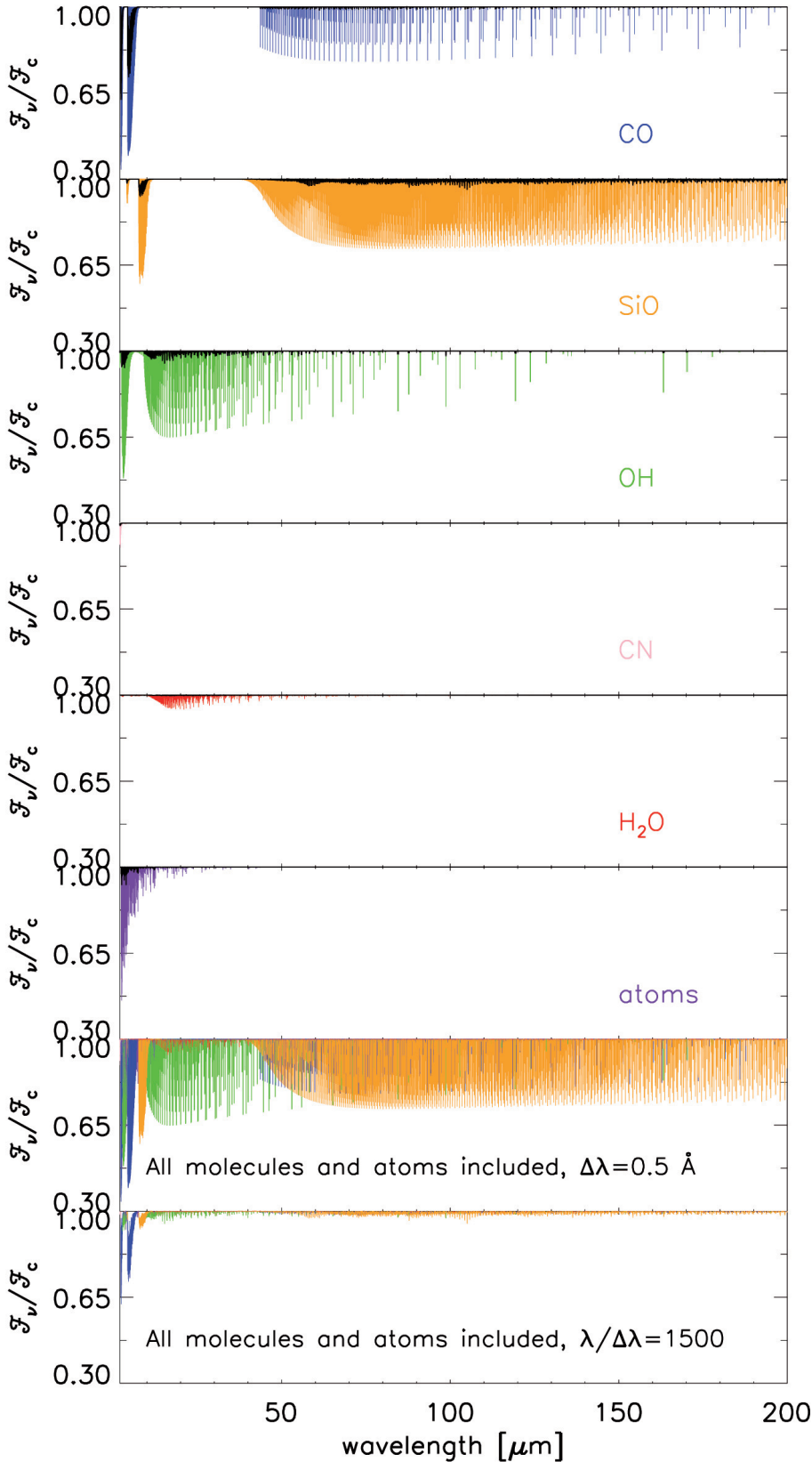
Fig. 7. Contribution of CO (blue), SiO (orange), OH (green), CN (pink), H 2 O (red), atoms (purple) to the 2–200 \mu\text{m} synthetic spectrum calculated from the atmosphere model with stellar parameters T_{\text{eff}} = 4320 K, \log g [ \text{cm/s}^2 ] = 1.50, mass M = 1.1 M_{\odot} , [\text{Fe}/\text{H}] = -0.50 , microturbulence \xi_t = 2 km s -1 , \varepsilon(\text{C}) = 7.96 , \varepsilon(\text{N}) = 7.61 , \varepsilon(\text{O}) = 8.68 , \varepsilon(\text{Mg}) = 7.33 , \varepsilon(\text{Si}) = 7.20 , and ^{12}\text{C}/^{13}\text{C} = 7 . The first six panels display the contribution at a resolution \Delta\lambda = 0.5 Å in color and at a medium resolution \lambda/\Delta\lambda = 1500 in black. The total contribution to the full spectrum is shown in the seventh panel at the high resolution of \Delta\lambda = 0.5 Å, and in the bottom panel at the medium resolution of \lambda/\Delta\lambda = 1500 . Note the lack of atomic absorption features for wavelengths longer than \sim 50 \mu\text{m} .
