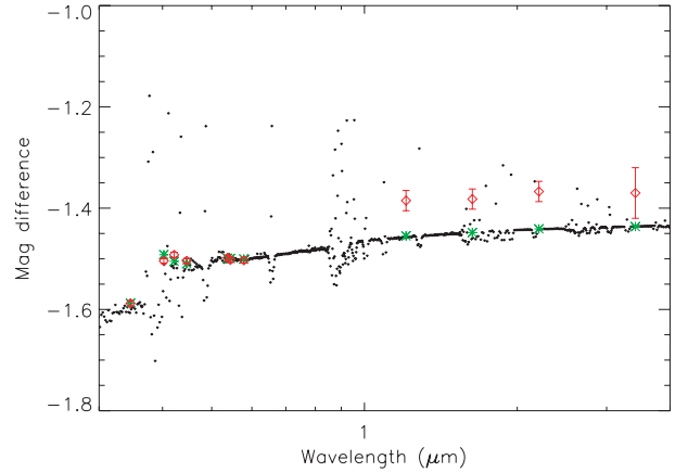
Fig. 3. Observed (red – diamonds) versus synthetic (green – stars) magnitude difference between Vega and Sirius ( \text{Mag}_{\text{Vega}} - \text{Mag}_{\text{Sirius}} ) in the Geneva photometric system and the JHKL bands (Verhoelst 2005). Black dotted line represents the difference between both of Kurucz’s models used in Cohen et al. (1992a), with stellar parameters T_{\text{eff}} = 9550\text{K} , \log g = 3.95 , [\text{Fe}/\text{H}] = -0.3 for Vega and T_{\text{eff}} = 9850\text{K} , \log g = 4.25 , [\text{Fe}/\text{H}] = +0.5 for Sirius. However, the Kurucz’s model for Sirius is scaled in such a way as to match the observed difference in the Geneva photometric system, yielding an angular diameter for Sirius of 6.15 mas (instead of 6.04 mas as used in Cohen et al. 1992a). Clearly, the (N)IR magnitude differences are not compatible as they differ by up to 10%.
