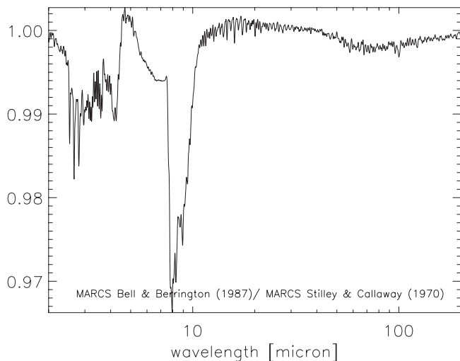
Fig. 9. Ratio between the synthetic spectrum calculated with the \text{H}_{\text{ff}}^- absorption coefficients of Bell & Berrington (1987) and the spectrum based on the \text{H}_{\text{ff}}^- absorption coefficients of Stille & Callaway (1970). The same stellar parameters as in Fig. 7 are used, data are reduced to a resolution of \lambda/\Delta\lambda = 100 .
