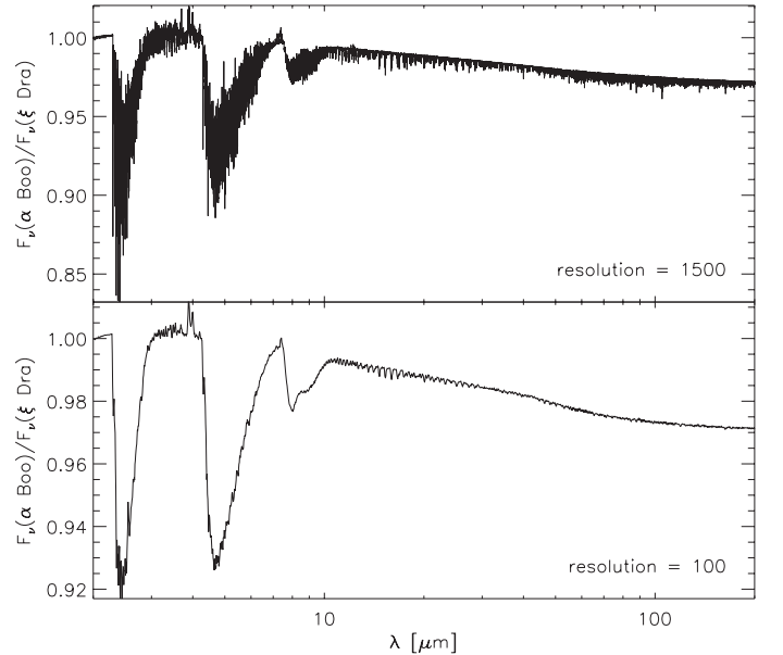
Fig. 12. Upper panel: comparison between the MARCS model spectrum of \alpha Boo and \xi Dra at a resolution of 1500. Both spectra have a fictitious angular diameter of 1 mas. Bottom panel: same as for the upper panel, but now at a resolution of 100. In regions of strong molecular absorption, the maximum difference is 15% for \lambda/\Delta\lambda = 1500 , and 8% for \lambda/\Delta\lambda = 100 .
