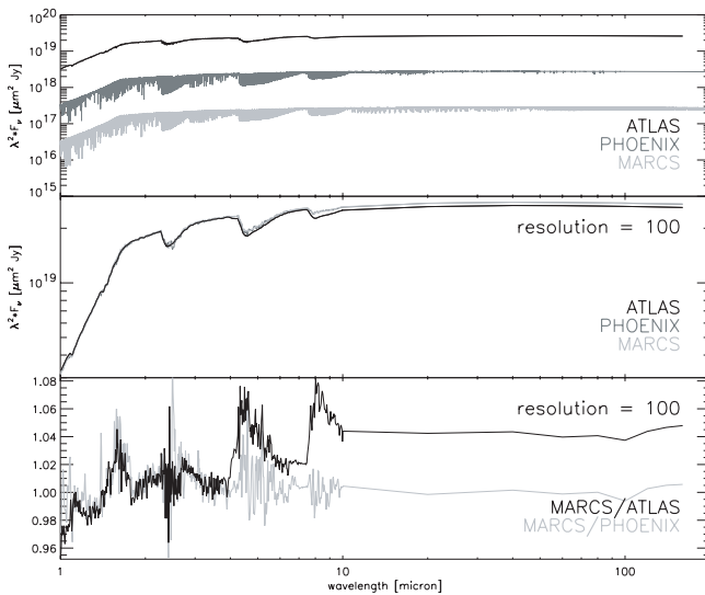
Fig. 6. Upper panel: comparison between the ATLAS, PHOENIX, and MARCS model spectra. The PHOENIX model is shifted downwards with a factor 10, and the MARCS model with a factor 100. Middle panel: comparison between the ATLAS, PHOENIX and MARCS model spectra at a resolution of 100 for \lambda \leq 10 \mu\text{m} . At longer wavelengths, only the 8 wavelength points as given in the ATLAS models (at 20, 40, 60, 80, 100, 120, 140, and 160 \mu\text{m} ) are retained. Difference between PHOENIX and MARCS model fluxes is barely visible. Bottom panel: ratio between MARCS and ATLAS (black) and PHOENIX (gray) model fluxes.
