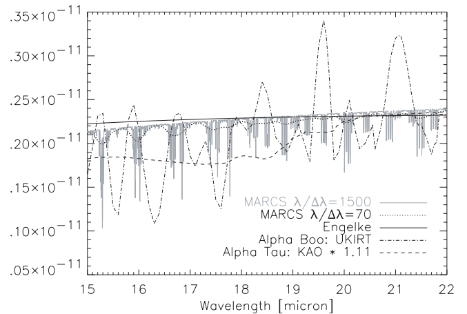
Fig. 4. UKIRT CGS3 15\text{--}22\mu\text{m} spectrum for \alpha Boo (K2 IIIp; unscaled, dash-dot line) and KAO spectrum for \alpha Tau (K5 III; scaled by a factor 1.11, dashed line) are compared with the Engelke approximation (full line) with parameters as used by Cohen et al. (1996b) for \alpha Boo ( T_{\text{eff}} = 4362\text{K} , \theta_d = 21.12\text{mas} ), and an appropriate theoretical MARCS model at a resolution \lambda/\Delta\lambda = 1500 (grey line) and at a resolution of \lambda/\Delta\lambda = 70 (dotted line; corresponding to the UKIRT CGS3 resolution), with stellar parameters as determined in Decin et al. (2003a).
