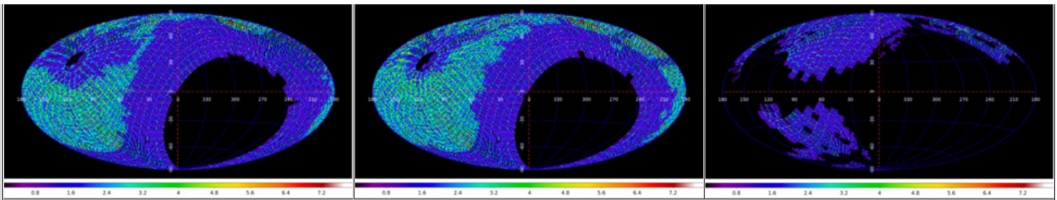
Figure 2 - Spatial distribution representing lightcurve (and \approx Reference Image) coverage in DR2, binned on approximate CCD-quadrant scales, in Galactic coordinates centered at l, b = 0, 0 . Left: g -filter; Center: r -filter; Right: i -filter. The color bar does not represent the number of observation epochs, but the number of neighboring CCD-quadrants that happen to overlap due to the fixed sky-tiling and coarse resampling of their centers on 1^\circ scales. Click on a panel to enlarge.
