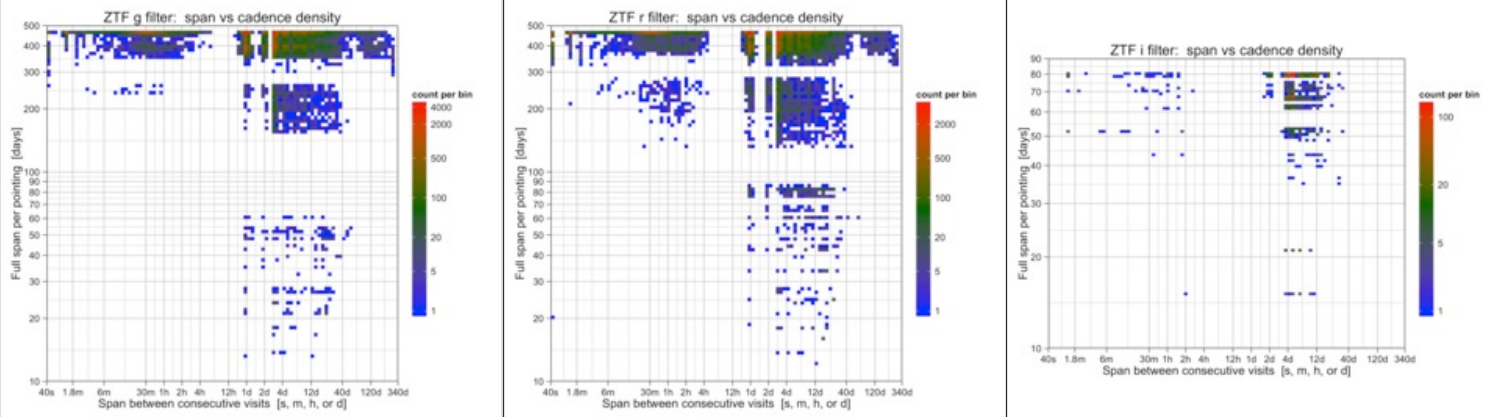
Figure 4 - Effective timespan per pointing (per \approx 7^\circ \times 7^\circ survey field) versus visit cadence. See text above for details. Left: g -filter; Center: r -filter; Right: i -filter. Click on a panel to enlarge.
