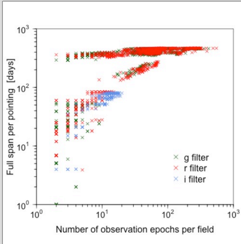
Figure 3 - Timespan of observations per survey-field as a function of the number of epochs in each. These timespans are proxies for the overall spans of lightcurves in DR2.
