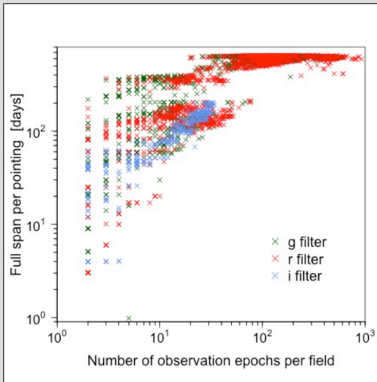
Figure 3 - Timespan of observations per survey-field as a function of the number of epochs in each. These timespans are proxies for the overall spans of lightcurves in DR3.
