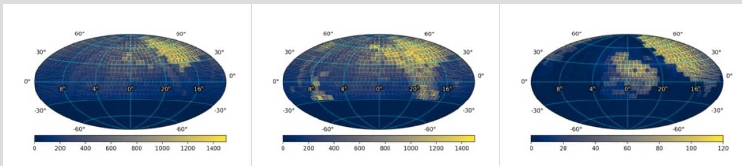
Figure 1 - Sky coverage and number of observation epochs per approximate CCD-quadrant footprint represented in DR5, in equatorial coordinates centered at ra, dec = 0, 0 . Left: g -filter; Center: r -filter; Right: i -filter. Color bar represents the number of observation epochs. Dark regions on small scales are not holes in coverage, but due to the coarse resampling of CCD-quadrant centers on 1^\circ scales. This resampling also distorts the true number of epochs per pointing (see Figure 3a for the true epoch distribution). Click on a panel to enlarge.
