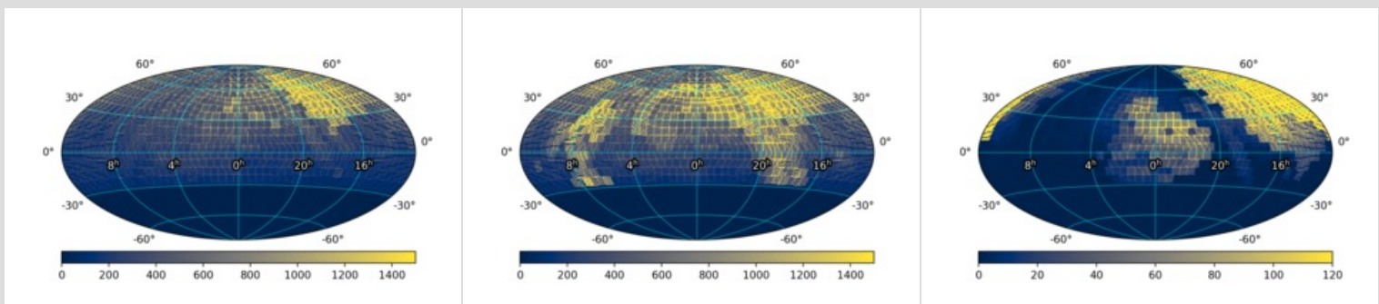
Figure 1 - Sky coverage and number of observation epochs per approximate CCD-quadrant footprint represented in DR8 in
