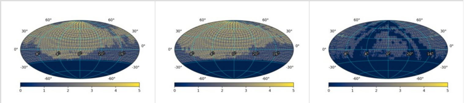
Figure 2 - Spatial distribution representing lightcurve (and \approx Reference Image) coverage in DR8, binned on approximate CCD-quadrant scales, in equatorial coordinates centered at ra, dec = 0, 0 . Left: g -filter; Center: r -filter; Right: i -filter. The color bar does not represent the number of observation epochs, but the number of neighboring CCD-quadrants that happen to overlap due to the fixed sky-tiling and coarse resampling of their centers on 1^\circ scales. Click on a panel to enlarge.
