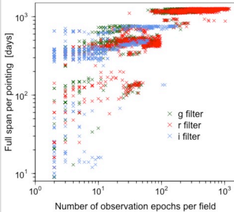
Figure 3 - Timespan of observations per survey-field as a function of the number of epochs in each. These timespans are proxies for the overall spans of lightcurves in DR8.
