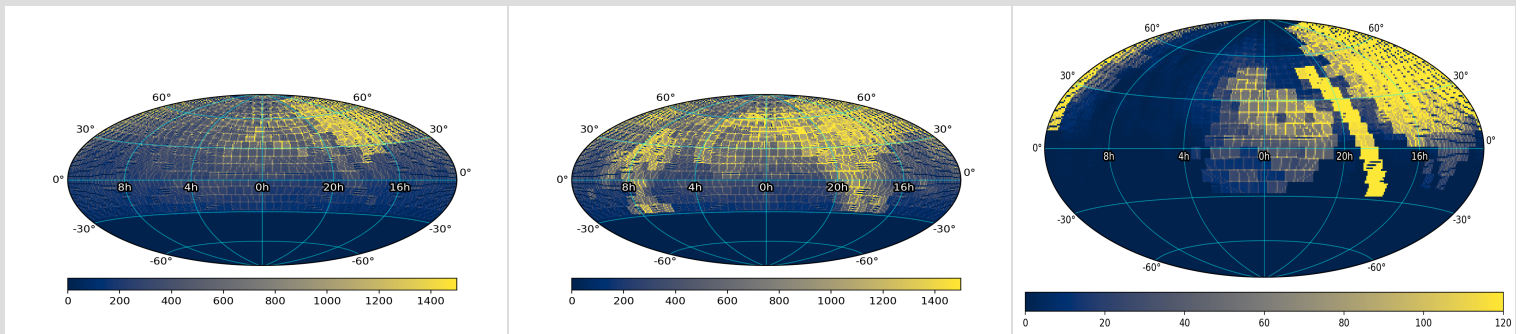
Figure 1 - Sky coverage and number of observation epochs per approximate CCD-quadrant footprint represented in DR10 in
