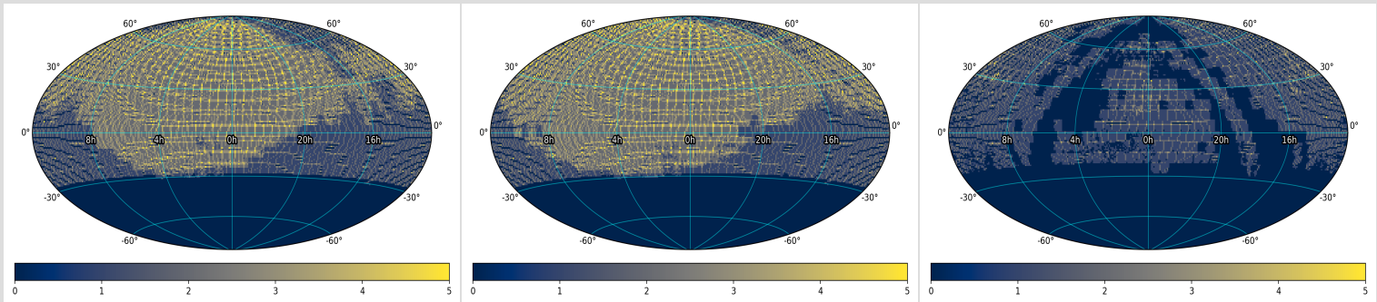
Figure 2 - Spatial distribution representing lightcurve (and \approx Reference Image) coverage in DR10, binned on approximate CCD-quadrant scales, in equatorial coordinates centered at ra, dec = 0, 0 . Left: g -filter; Center: r -filter; Right: i -filter. The color bar does not represent the number of observation epochs, but the number of neighboring CCD-quadrants that happen to overlap due to the fixed sky-tiling and coarse resampling of their centers on 1^\circ scales. Click on a panel to enlarge.
