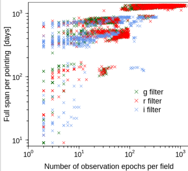
Figure 3 - Timespan of observations per survey-field as a function of the number of epochs in each. These timespans are proxies for the overall spans of lightcurves in DR10.
