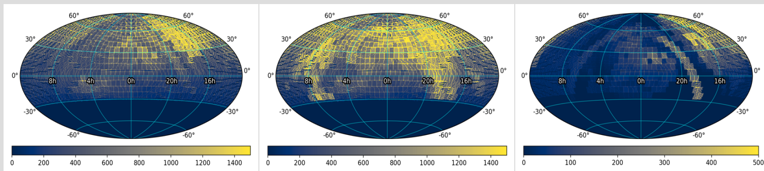
Figure 1 - Sky coverage and number of observation epochs per approximate CCD-quadrant footprint represented in DR13 in equatorial coordinates centered at ra, dec = 0, 0 . Left: g -filter; Center: r -filter; Right: i -filter. Color bar represents the number of observation epochs. Dark regions on small scales are not holes in coverage, but due to the coarse resampling of CCD-quadrant centers on 1^\circ scales. This resampling also distorts the true number of epochs per pointing (see Figure 3a for the true epoch distribution). Click on a panel to enlarge.
