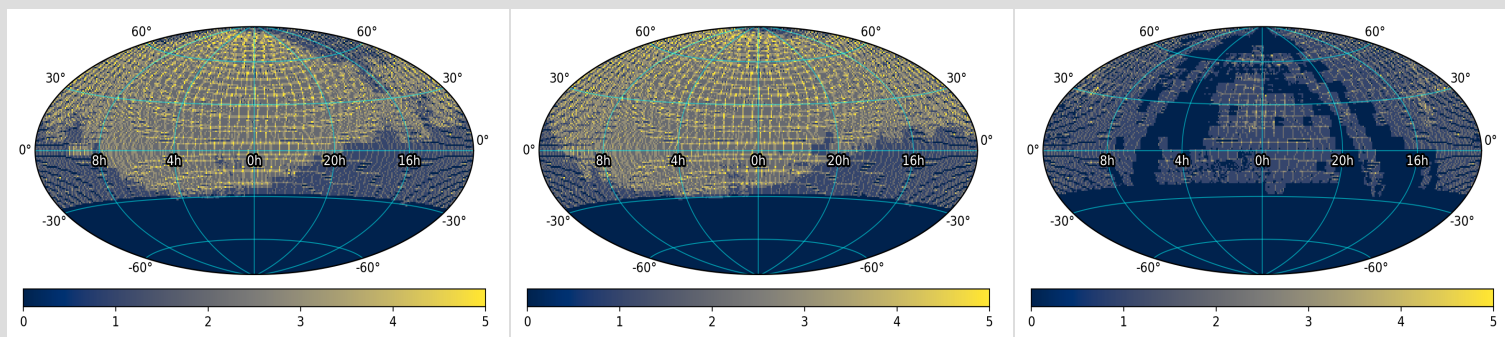
Figure 2 - Spatial distribution representing lightcurve (and \approx Reference Image) coverage in DR13, binned on approximate CCD-quadrant scales, in equatorial coordinates centered at ra, dec = 0, 0 . Left: g -filter; Center: r -filter; Right: i -filter. The color bar does not represent the number of observation epochs, but the number of neighboring CCD-quadrants that happen to overlap due to the fixed sky-tiling and coarse resampling of their centers on 1^\circ scales. Click on a panel to enlarge.
