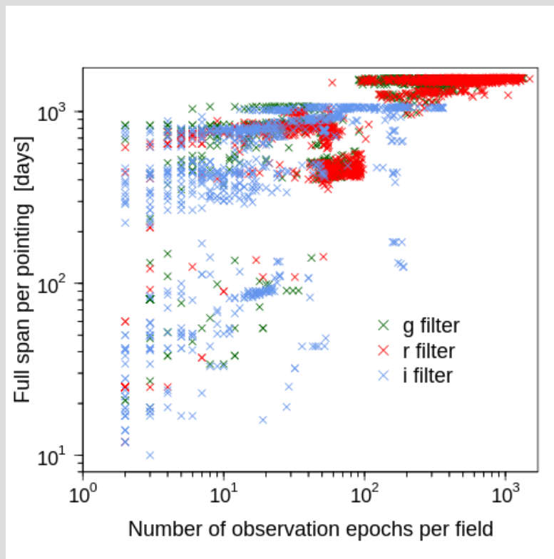
Figure 3 - Timespan of observations per survey-field as a function of the number of epochs in each. These timespans are proxies for the overall spans of lightcurves in DR13.
