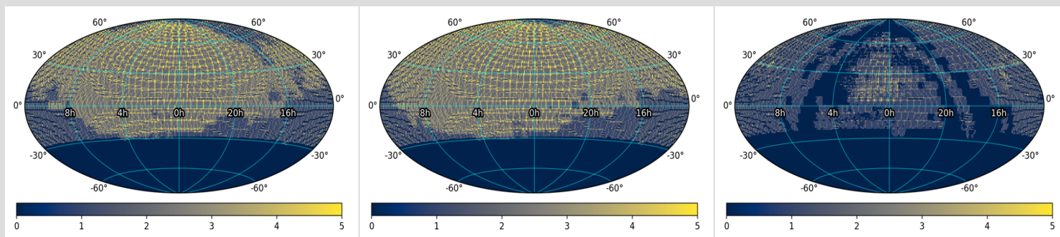
Figure 2 - Spatial distribution representing lightcurve (and \approx Reference Image) coverage in DR14, binned on approximate CCD-quadrant scales, in equatorial coordinates centered at ra, dec = 0, 0 . Left: g -filter; Center: r -filter; Right: i -filter. The color bar does not represent the number of observation epochs, but the number of neighboring CCD-quadrants that happen to overlap due to the fixed sky-tiling and coarse resampling of their centers on 1^\circ scales. Click on a panel to enlarge.
