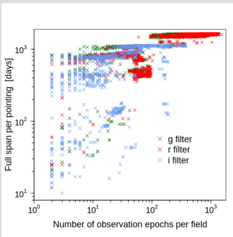
Figure 3 - Timespan of observations per survey-field as a function of the number of epochs in each. These timespans are proxies for the overall spans of lightcurves in DR14.
