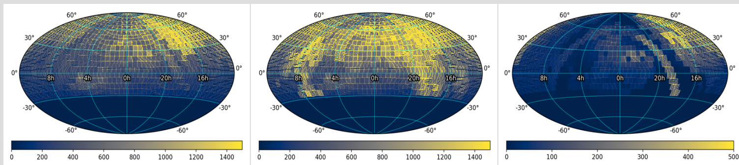
Figure 1 - Sky coverage and number of observation epochs per approximate CCD-quadrant footprint represented in DR14 in equatorial coordinates centered at ra, dec = 0, 0 . Left: g -filter; Center: r -filter; Right: i -filter. Color bar represents the number of observation epochs. Dark regions on small scales are not holes in coverage, but due to the coarse resampling of CCD-quadrant centers on 1^\circ scales. This resampling also distorts the true number of epochs per pointing (see Figure 3a for the true epoch distribution). Click on a panel to enlarge.
