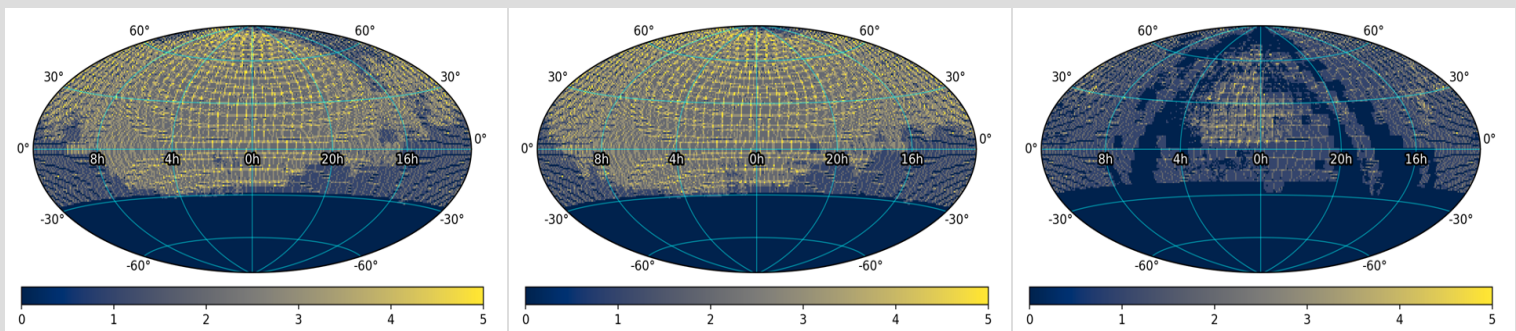
Figure 2 - Spatial distribution representing lightcurve (and \approx Reference Image) coverage in DR15, binned on approximate CCD-quadrant scales, in equatorial coordinates centered at ra, dec = 0, 0 . Left: g -filter; Center: r -filter; Right: i -filter. The color bar does not represent the number of observation epochs, but the number of neighboring CCD-quadrants that happen to overlap due to the fixed sky-tiling and coarse resampling of their centers on 1^\circ scales. Click on a panel to enlarge.
