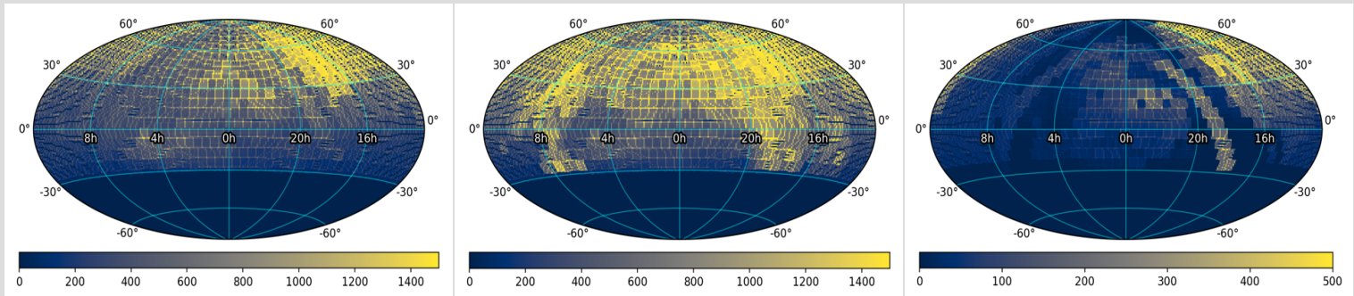
Figure 1 - Sky coverage and number of observation epochs per approximate CCD-quadrant footprint represented in DR15 in equatorial coordinates centered at ra, dec = 0, 0 . Left: g -filter; Center: r -filter; Right: i -filter. Color bar represents the number of observation epochs. Dark regions on small scales are not holes in coverage, but due to the coarse resampling of CCD-quadrant centers on 1^\circ scales. This resampling also distorts the true number of epochs per pointing (see Figure 3a for the true epoch distribution). Click on a panel to enlarge.
