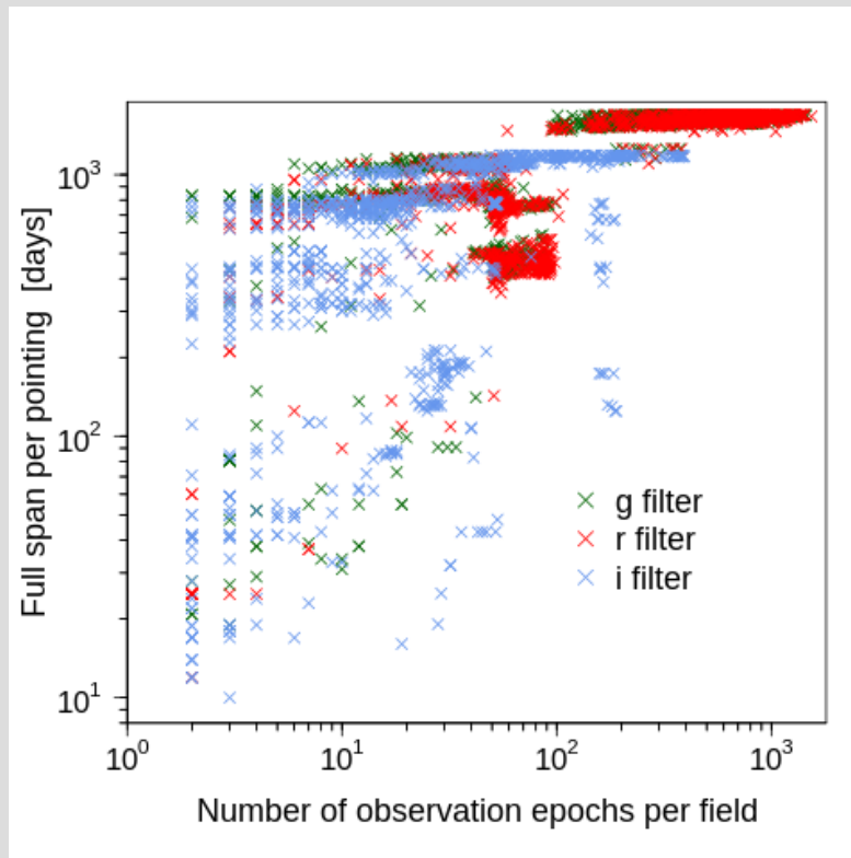
Figure 3 - Timespan of observations per survey-field as a function of the number of epochs in each. These timespans are proxies for the overall spans of lightcurves in DR15.
