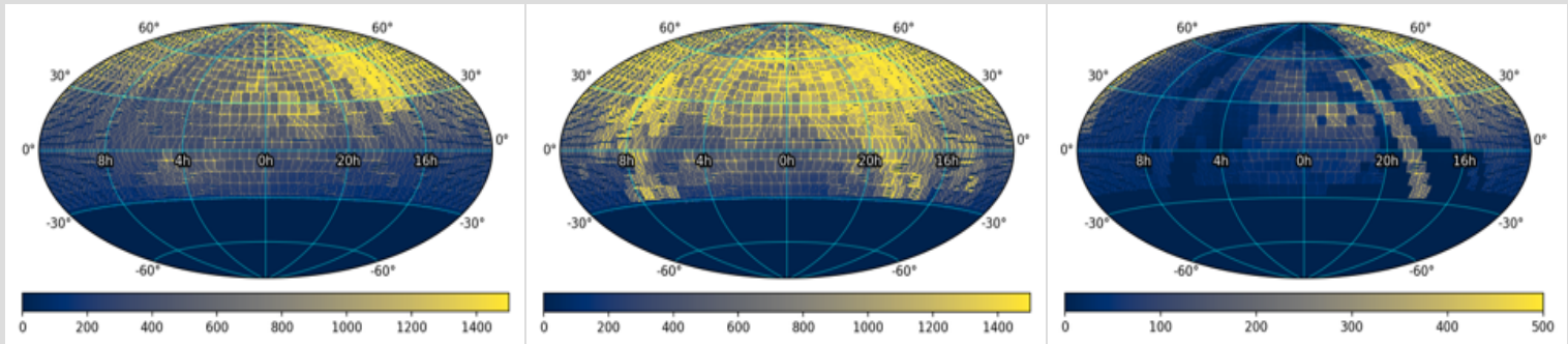
Figure 1 - Sky coverage and number of observation epochs per approximate CCD-quadrant footprint represented in DR16 in equatorial coordinates centered at ra, dec = 0, 0 . Left: g -filter; Center: r -filter; Right: i -filter. Color bar represents the number of observation epochs. Dark regions on small scales are not holes in coverage, but due to the coarse resampling of CCD-quadrant centers on 1^\circ scales. This resampling also distorts the true number of epochs per pointing (see Figure 3a for the true epoch distribution). Click on a panel to enlarge.
