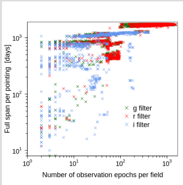
Figure 3 - Timespan of observations per survey-field as a function of the number of epochs in each. These timespans are proxies for the overall spans of lightcurves in DR16.
