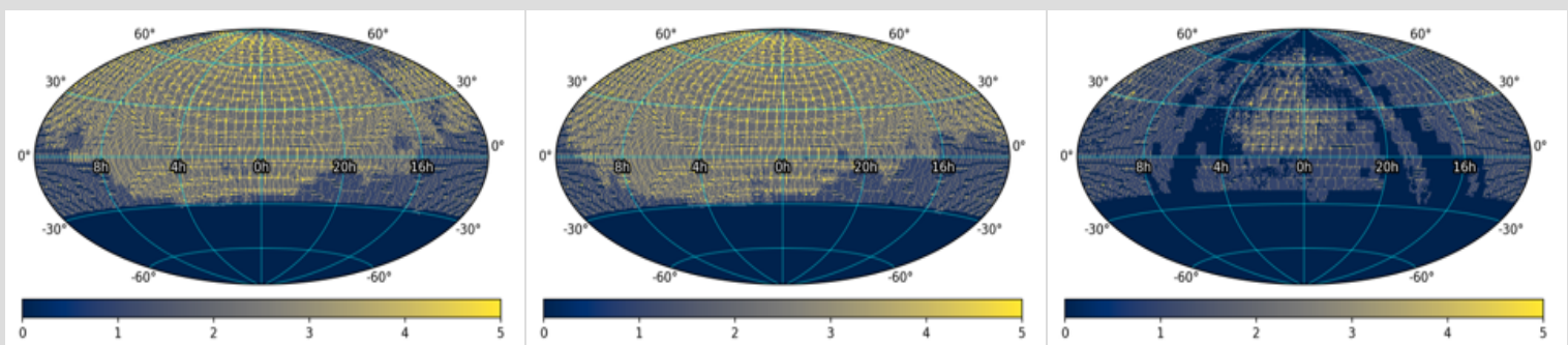
Figure 2 - Spatial distribution representing lightcurve (and \approx Reference Image) coverage in DR16, binned on approximate CCD-quadrant scales, in equatorial coordinates centered at ra, dec = 0, 0 . Left: g -filter; Center: r -filter; Right: i -filter. The color bar does not represent the number of observation epochs, but the number of neighboring CCD-quadrants that happen to overlap due to the fixed sky-tiling and coarse resampling of their centers on 1^\circ scales. Click on a panel to enlarge.
