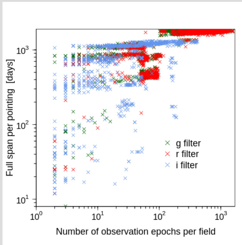
Figure 3 - Timespan of observations per survey-field as a function of the number of epochs in each. These timespans are proxies for the overall spans of lightcurves in DR17.
