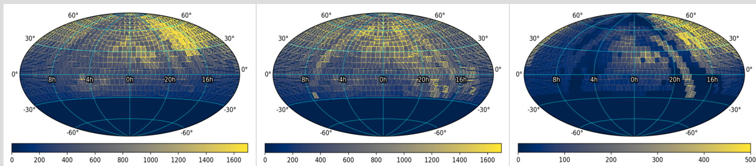
Figure 1 - Sky coverage and number of observation epochs per approximate CCD-quadrant footprint represented in DR17 in equatorial coordinates centered at ra, dec = 0, 0 . Left: g -filter; Center: r -filter; Right: i -filter. Color bar represents the number of observation epochs. Dark regions on small scales are not holes in coverage, but due to the coarse resampling of CCD-quadrant centers on 1^\circ scales. This resampling also distorts the true number of epochs per pointing (see Figure 3a for the true epoch distribution). Click on a panel to enlarge.
