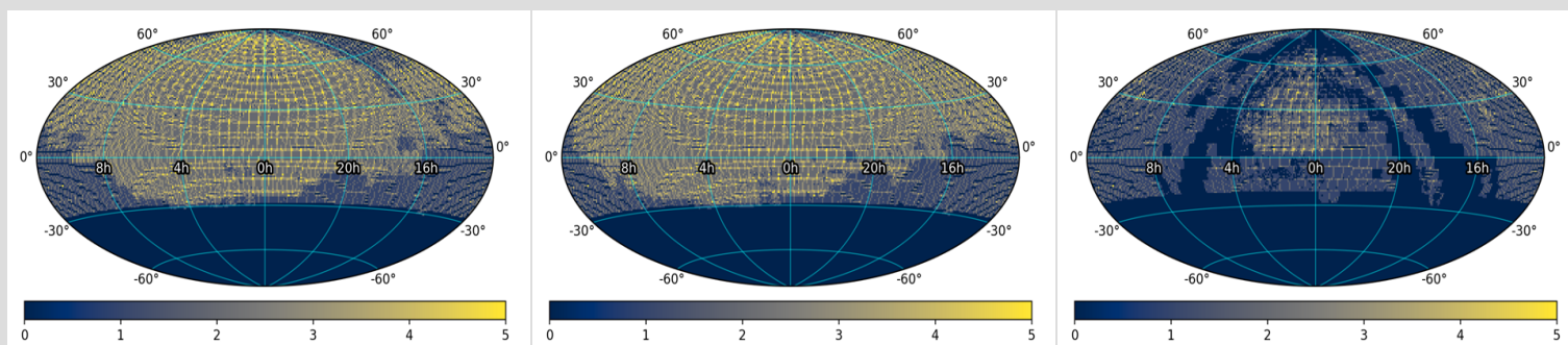
Figure 2 - Spatial distribution representing lightcurve (and \approx Reference Image) coverage in DR17, binned on approximate CCD-quadrant scales, in equatorial coordinates centered at ra, dec = 0, 0 . Left: g -filter; Center: r -filter; Right: i -filter. The color bar does not represent the number of observation epochs, but the number of neighboring CCD-quadrants that happen to overlap due to the fixed sky-tiling and coarse resampling of their centers on 1^\circ scales. Click on a panel to enlarge.
