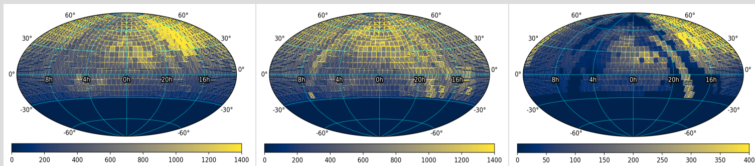
Figure 1 - Sky coverage and number of observation epochs per approximate CCD-quadrant footprint represented in DR19 in equatorial coordinates centered at ra, dec = 0, 0 . Left: g -filter; Center: r -filter; Right: i -filter. Color bar represents the number of observation epochs. Dark regions on small scales are not holes in coverage, but due to the coarse resampling of CCD-quadrant centers on 1^\circ scales. This resampling also distorts the true number of epochs per pointing (see Figure 3a for the true epoch distribution). Click on a panel to enlarge.
