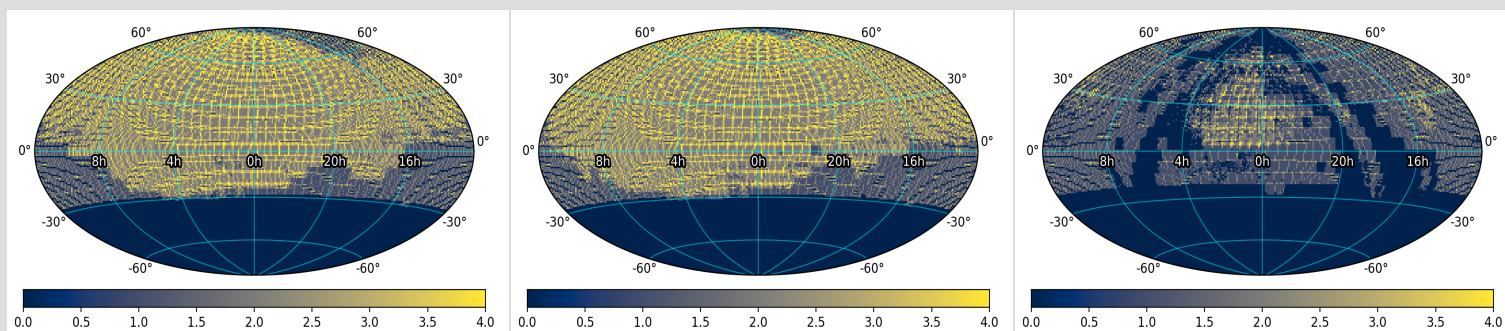
Figure 2 - Spatial distribution representing lightcurve (and \approx Reference Image) coverage in DR19, binned on approximate CCD-quadrant scales, in equatorial coordinates centered at ra, dec = 0, 0 . Left: g -filter; Center: r -filter; Right: i -filter. The color bar does not represent the number of observation epochs, but the number of neighboring CCD-quadrants that happen to overlap due to the fixed sky-tiling and coarse resampling of their centers on 1^\circ scales. Click on a panel to enlarge.
