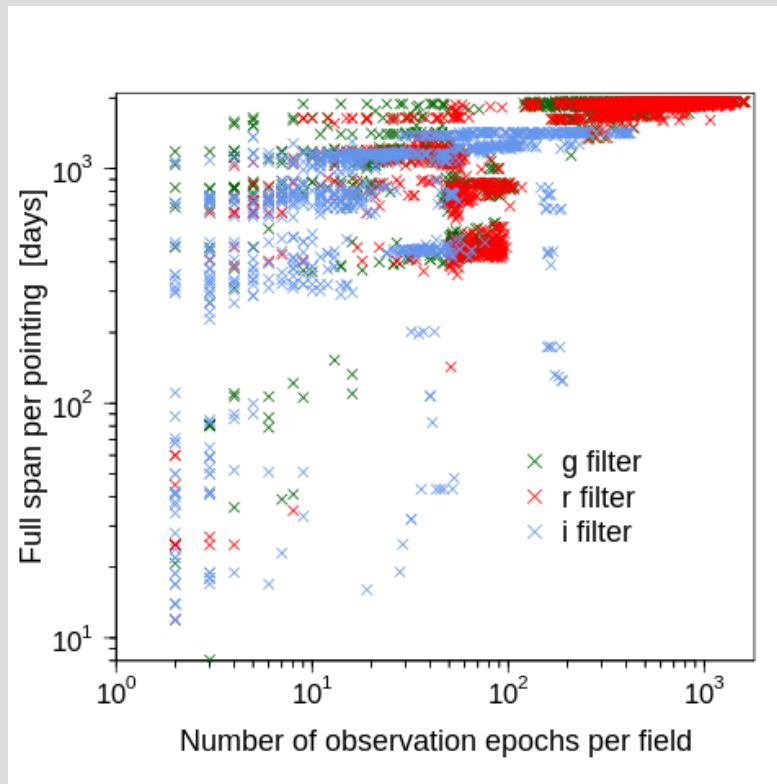
Figure 3 - Timespan of observations per survey-field as a function of the number of epochs in each. These timespans are proxies for the overall spans of lightcurves in DR19.
