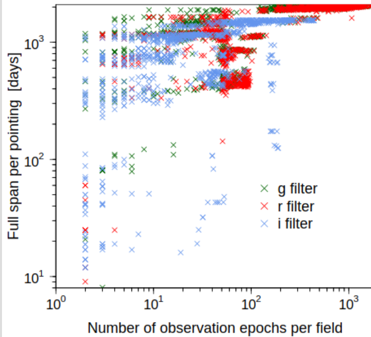
Figure 3 - Timespan of observations per survey-field as a function of the number of epochs in each. These timespans are proxies for the overall spans of lightcurves in DR20.
