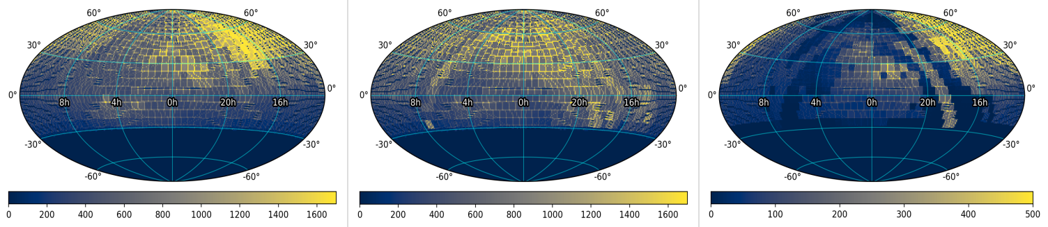
Figure 1 - Sky coverage and number of observation epochs per approximate CCD-quadrant footprint represented in DR20 in equatorial coordinates centered at ra, dec = 0, 0 . Left: g -filter; Center: r -filter; Right: i -filter. Color bar represents the number of observation epochs. Dark regions on small scales are not holes in coverage, but due to the coarse resampling of CCD-quadrant centers on 1^\circ scales. This resampling also distorts the true number of epochs per pointing (see Figure 3a for the true epoch distribution). Click on a panel to enlarge.
