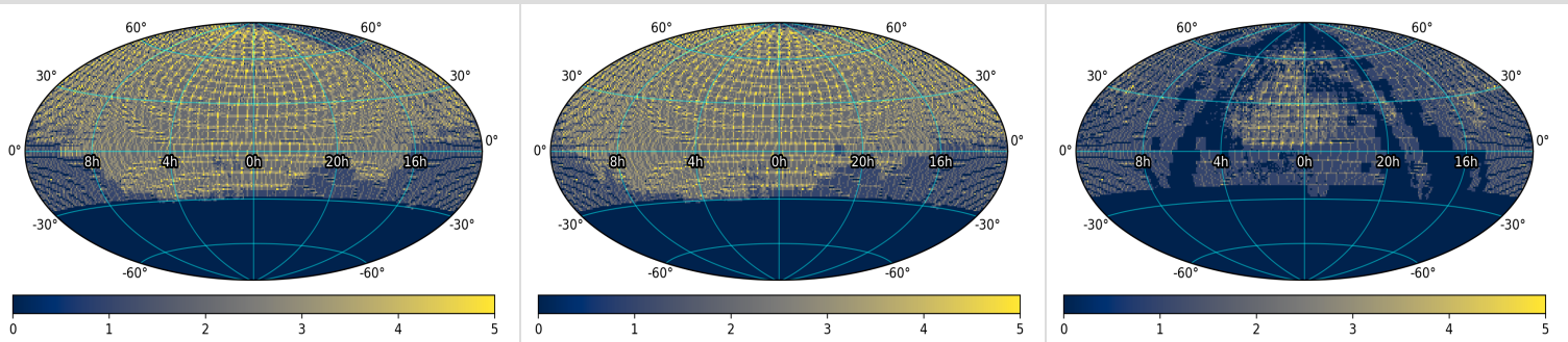
Figure 2 - Spatial distribution representing lightcurve (and \approx Reference Image) coverage in DR20, binned on approximate CCD-quadrant scales, in equatorial coordinates centered at ra, dec = 0, 0 . Left: g -filter; Center: r -filter; Right: i -filter. The color bar does not represent the number of observation epochs, but the number of neighboring CCD-quadrants that happen to overlap due to the fixed sky-tiling and coarse resampling of their centers on 1^\circ scales. Click on a panel to enlarge.
