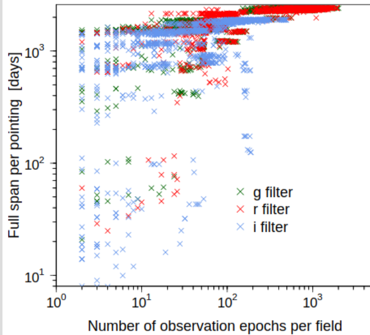
Figure 3 - Timespan of observations per survey-field as a function of the number of epochs in each. These timespans are proxies for the overall spans of lightcurves in DR23.
