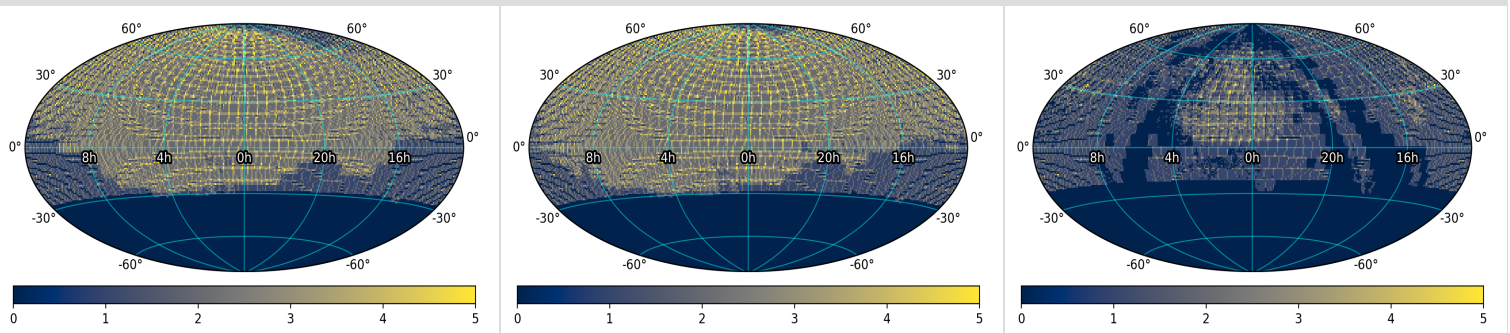
Figure 2 - Spatial distribution representing lightcurve (and \approx Reference Image) coverage in DR23, binned on approximate CCD-quadrant scales, in equatorial coordinates centered at ra, dec = 0, 0 . Left: g -filter; Center: r -filter; Right: i -filter. The color bar does not represent the number of observation epochs, but the number of neighboring CCD-quadrants that happen to overlap due to the fixed sky-tiling and coarse resampling of their centers on 1^\circ scales. Click on a panel to enlarge.
