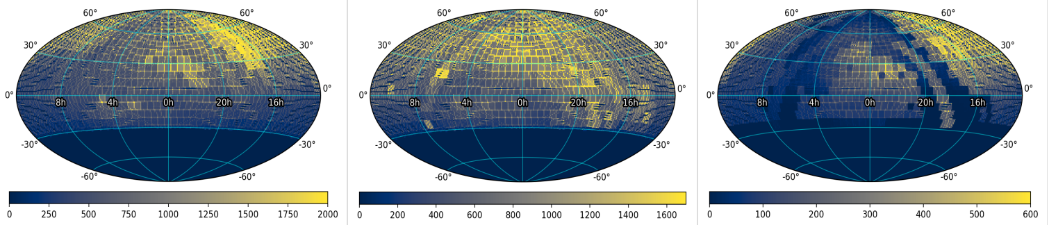
Figure 1 - Sky coverage and number of observation epochs per approximate CCD-quadrant footprint represented in DR23 in equatorial coordinates centered at ra, dec = 0, 0 . Left: g -filter; Center: r -filter; Right: i -filter. Color bar represents the number of observation epochs. Dark regions on small scales are not holes in coverage, but due to the coarse resampling of CCD-quadrant centers on 1^\circ scales. This resampling also distorts the true number of epochs per pointing (see Figure 3a for the true epoch distribution). Click on a panel to enlarge.
