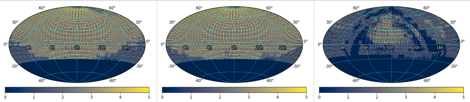
Figure 2 - Spatial distribution representing lightcurve (and \approx Reference Image) coverage in DR24, binned on approximate CCD-quadrant scales, in equatorial coordinates centered at ra, dec = 0, 0 . Left: g -filter; Center: r -filter; Right: i -filter. The color bar does not represent the number of observation epochs, but the number of neighboring CCD-quadrants that happen to overlap due to the fixed sky-tiling and coarse resampling of their centers on 1^\circ scales. Click on a panel to enlarge.
