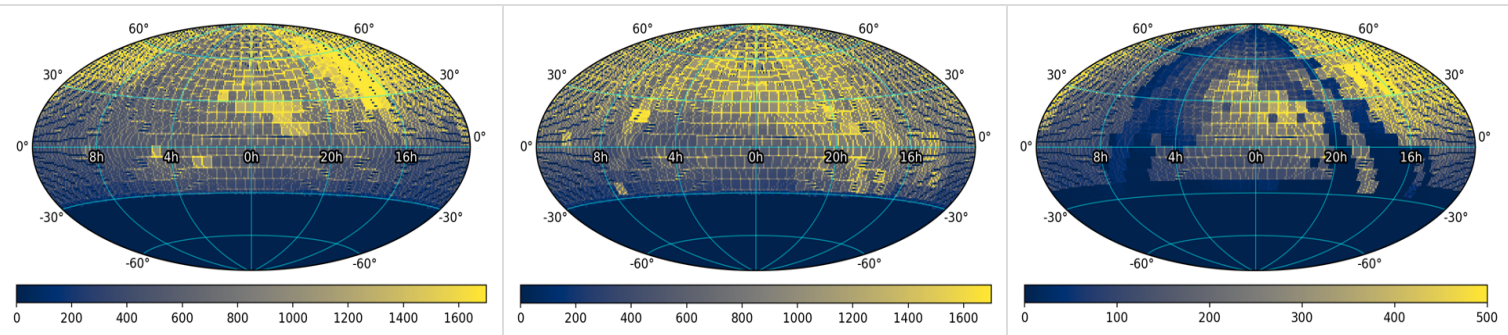
Figure 1 - Sky coverage and number of observation epochs per approximate CCD-quadrant footprint represented in DR24 in equatorial coordinates centered at ra, dec = 0, 0 . Left: g -filter; Center: r -filter; Right: i -filter. Color bar represents the number of observation epochs. Dark regions on small scales are not holes in coverage, but due to the coarse resampling of CCD-quadrant centers on 1^\circ scales. This resampling also distorts the true number of epochs per pointing (see Figure 3a for the true epoch distribution). Click on a panel to enlarge.
