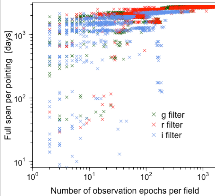
Figure 3 - Timespan of observations per survey-field as a function of the number of epochs in each. These timespans are proxies for the overall spans of lightcurves in DR24.
