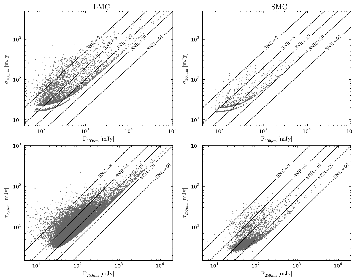
Fig. 24.— PACS 100 \mu\text{m} (top row) and SPIRE 250 \mu\text{m} (bottom row) catalog source flux uncertainty as a function of flux for the LMC (left), and SMC (right). Lines of constant SNR are drawn to guide the eye.
