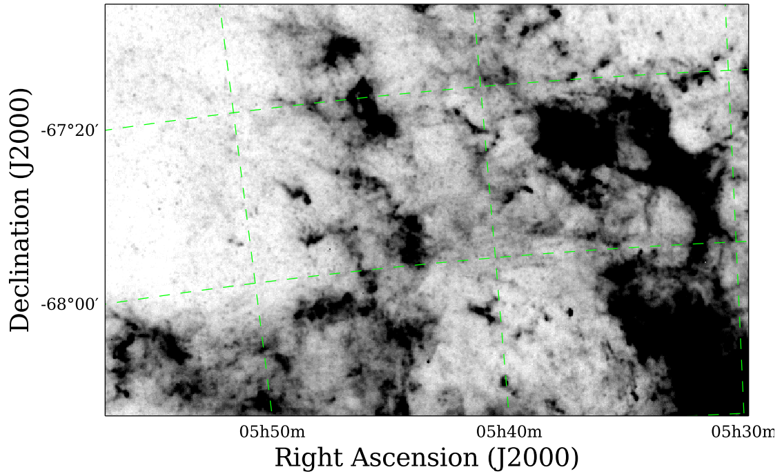
Fig. 11.— Top panel: a section of the SPIRE 500 \mu\text{m} band map of the LMC produced with the standard HIPE 7 pipeline. The vertical and horizontal stripes are due to residuals left by temperature drift correction during strong temperature variations (see Section 4). Bottom panel: same region as in the top panel of the SPIRE 500 \mu\text{m} band map produced using new temperature drift coefficients.
