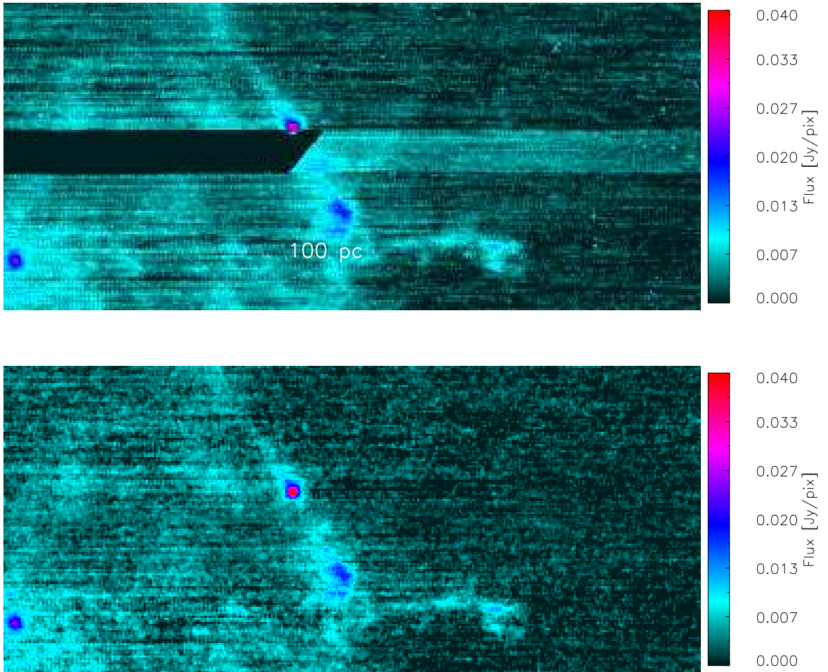
Fig. 5.— Example of a long glitch, a cosmic ray hit affecting an entire line of bolometers in the PACS 100\ \mu\text{m} detector. The top panel shows the image of the glitch, while the bottom panel shows the projected timelines after the long glitch has been removed by our custom algorithm.
