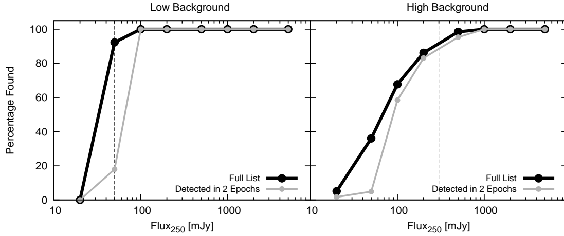
Fig. 25.— Completeness curves for SPIRE 250 \mu\text{m} created from the false source injection test, which show the percentage of false sources recovered as a function of flux. The left and right panels are for sources within a low ( \leq 10 MJy/sr) and high ( > 10 MJy/sr) background, respectively. The black curve is for all sources recovered from the combined image (i.e. the Full List), while the grey curve is Full List sources detected in both individual epoch images. The vertical lines mark the Full List 90% completeness limit at each background level.
