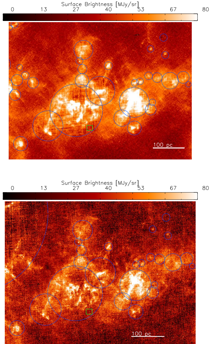
Fig. 10.— Zoom-in on the PACS 160 (top) and 100 (bottom) \mu\text{m} maps of the LMC. The blue circles correspond to masks used to estimate the 1/f noise and bolometer drifts (section 3.5, Figure 4). The green box shows an example of region used to estimate the residual noise in masked regions of the LMC.
