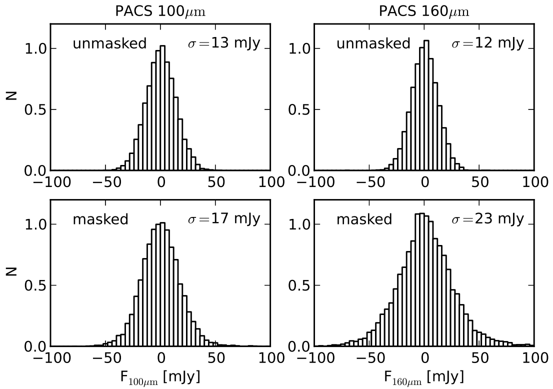
Fig. 23.— The same as Figure 22, but for the SMC.
