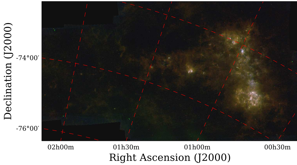
Fig. 16.— The SMC HERITAGE data. Red corresponds to SPIRE 250 \mu\text{m} , green to PACS 160 \mu\text{m} , and blue to PACS 100 \mu\text{m} .
