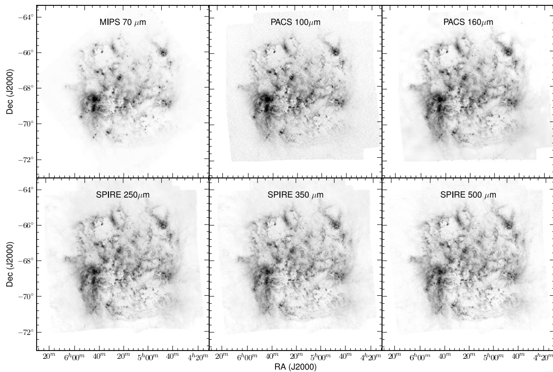
Fig. 13.— The HERITAGE data for the LMC with the Spitzer -SAGE-LMC MIPS 70 \mu\text{m} image (Meixner et al. 2006) for comparison. Together these data sets sample the spectral energy distribution of ISM dust emission. The grey scale displays are all in arcsinh with the following ranges: MIPS 70 \mu\text{m} , 0–400 MJy sr ^{-1} ; PACS 100 \mu\text{m} , 0–400 MJy sr ^{-1} ; PACS 160 \mu\text{m} , 5–500 MJy sr ^{-1} ; SPIRE 250 \mu\text{m} , 1–300 MJy sr ^{-1} ; SPIRE 350 \mu\text{m} , 0–170 MJy sr ^{-1} ; SPIRE 500 \mu\text{m} , 0–70 MJy sr ^{-1} .
