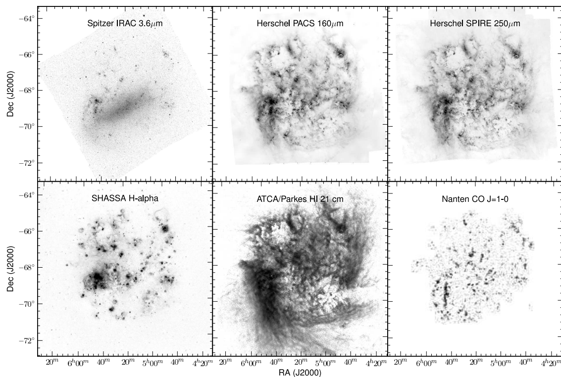
Fig. 17.— LMC survey data. From top to bottom, left to right: The Spitzer IRAC 3.6 \mu\text{m} image from the SAGE-LMC survey (Meixner et al. 2006) reveals the old stellar population, which is ejecting dust into the ISM. The Herschel PACS 160 \mu\text{m} and SPIRE 250 \mu\text{m} image from the HERITAGE survey reveal the coolest dust emission, which is dominated by the larger dust grains. The \text{H}\alpha emission from SHASSA (Gaustad et al. 2001) shows the distribution of the diffuse ionized gas, punctuated by \text{H II} regions. The \text{H I} 21 cm emission (Kim et al. 2003) show the location of the atomic neutral hydrogen. The \text{CO J}=1-0 emission survey by NANTEN (Fukui et al. 2008) traces the highest column density of molecular gas. The grey scale displays are all in arcsinh with the following ranges: IRAC 3.6 \mu\text{m} 0–5 \text{MJy sr}^{-1} ; PACS 160 \mu\text{m} 5–500 \text{MJy sr}^{-1} ; SPIRE 250 \mu\text{m} -1–300 \text{MJy sr}^{-1} ; \text{H}\alpha 0–8000 ; \text{H I} 21 cm, 4–70 10^{20} \text{ cm}^{-2} ; \text{CO J}=1-0 , 0–15 \text{K km/s} .
