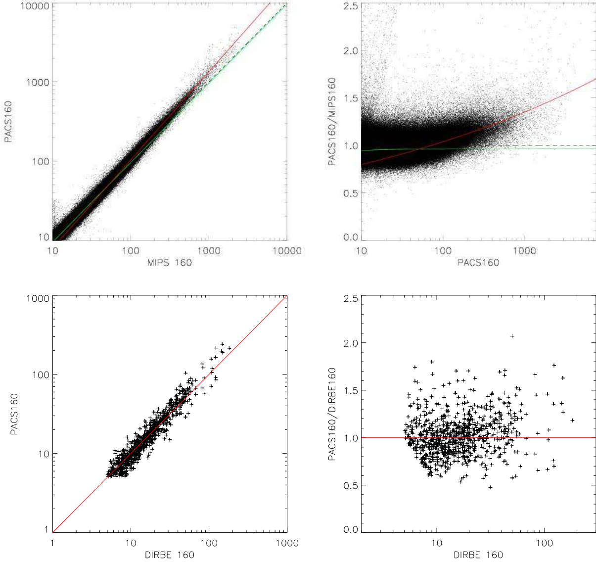
Fig. 8.— Pixel-to-pixel surface brightness correlation between the combined epochs of the PACS 160 \mu\text{m} convolved, resampled images of the LMC, and the MIPS 160 \mu\text{m} on the one hand (top), and the interpolation at 160 \mu\text{m} between the DIRBE 140 and 240 \mu\text{m} bands on the other hand (bottom). Surface brightnesses are plotted in MJy/sr. In the top panel, the green line shows a bisector linear fit, of slope 0.96, to the correlation in the linear range of the MIPS detector (surface brightness below 50 MJy/sr). The red line shows an exponential fit to the correlation in the non-linear range of MIPS (surface brightness above 50 MJy/sr), which yields (\text{PACS}/50 \text{ MJy/sr}) = 0.96 (\text{MIPS}/50 \text{ MJy/sr})^{1.11} in the non-linear regime. In the bottom panel, the red line shows a 1:1 correlation.
