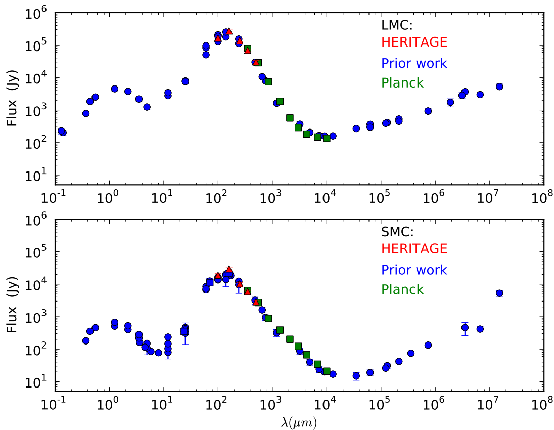
Fig. 19.— The spectral energy distributions of the whole LMC and SMC cover the UV to radio wavelengths. Prior work summarized by Israel et al. (2010) includes data from ground and space based missions such as IRAS, DIRBE, TopHat and WMAP. For the SMC, we also include prior work (blue squares) from Gordon et al. (2011). The HERITAGE photometry measured in the PACS and SPIRE bands are shown in red. The Planck measurements are shown in green (Planck collaboration 2011).
