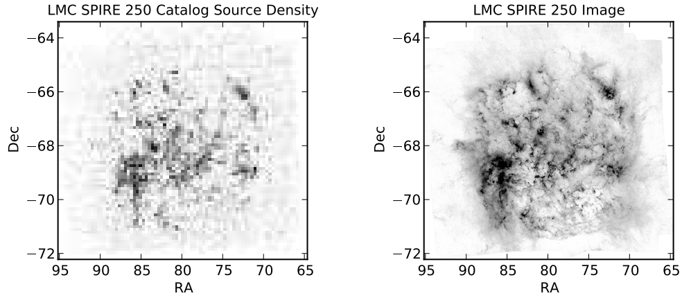
Fig. 28.— Left: The LMC’s spatial distribution of the 250\ \mu\text{m} catalog sources shown as a source density plot where the greyscale is linear with a range from 0 to 40 sources per pixel, where the pixel is 6.6' or 100 pc on a side. Right: Comparison to the SPIRE 250\ \mu\text{m} image shown in grey scale with a square root stretch and a flux range of 0 to 100 MJy/sr.
