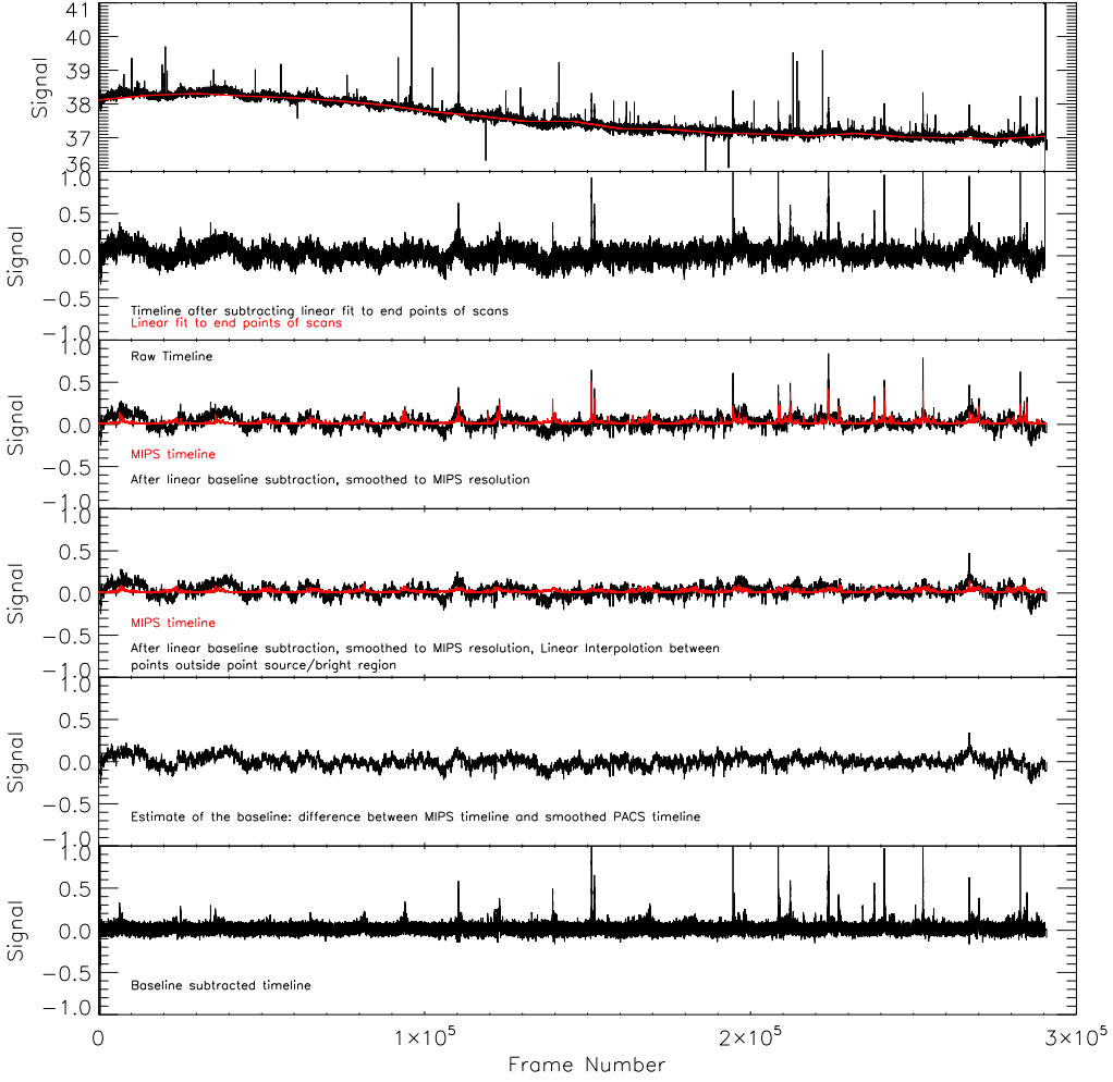
Fig. 2.— PACS timelines for one bolometer and during one AOR, at the different steps of the PACS processing algorithm. Starting from the top, the first panel shows the raw timeline in black, on which is over-plotted in red the linear fit to the end points of each scan leg, performed during the rough baseline estimate. The second panel shows the timeline resulting from this rough baseline subtraction. The third panel shows the timeline after initial rough baseline subtraction, smoothed to MIPS resolution using a 1D slice through the center of the 2D convolution kernel in black. The synthetic MIPS timeline obtained from the PACS mapping scheme and the MIPS map is shown in red. The fourth panel shows the MIPS timeline in red, and in black, the PACS timeline, after a rough baseline subtraction, smoothed to MIPS resolution, and after performing a linear interpolation inside masked bright and/or compact regions. The fifth panel shows the final estimation of the residual baseline (i.e., after rough baseline removal from a linear fit to the end points of each scan leg), obtained by subtracting the MIPS timeline to the smoothed, interpolated PACS timeline in the fourth panel. The final, baseline subtracted PACS timeline is shown in the bottom panel.
