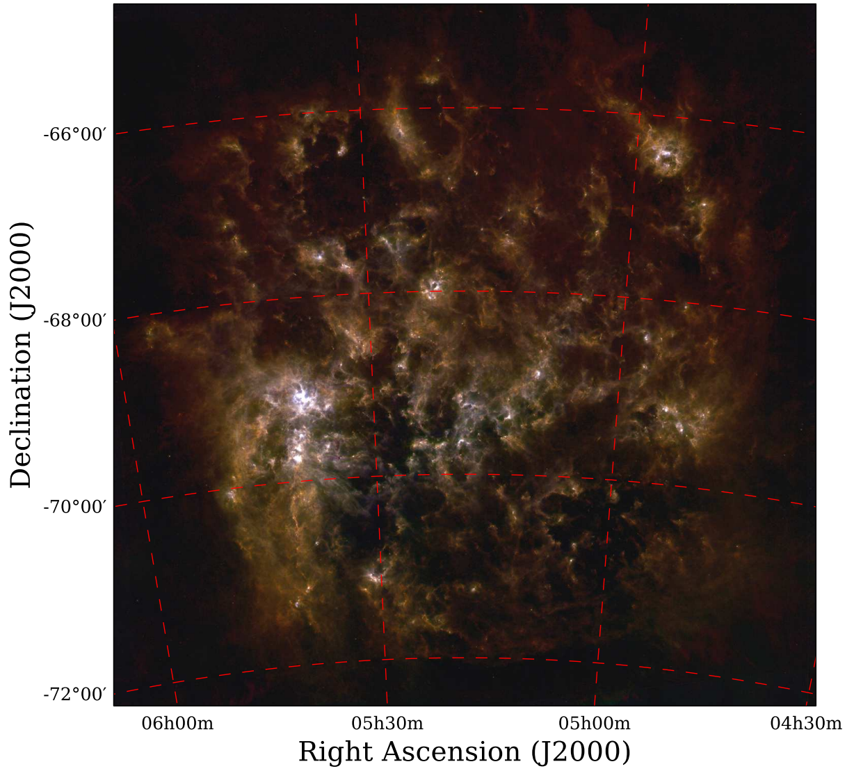
Fig. 14.— The LMC HERITAGE data. Red corresponds to SPIRE 250 \mu\text{m} , green to PACS 160 \mu\text{m} , and blue to PACS 100 \mu\text{m} .
