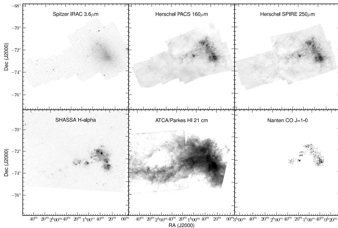
Fig. 18.— The same type of survey data as Figure 17 but from different sources, for the SMC. The Spitzer IRAC 3.6 \mu\text{m} image from the SAGE-SMC survey (Gordon et al. 2011) reveals the old stellar population. The Herschel PACS 160 \mu\text{m} and SPIRE 250 \mu\text{m} images from the HERITAGE survey reveal the coolest dust emission. The \text{H}\alpha emission from SHASSA (Gaustad et al. 2001) shows the distribution of the diffuse ionized gas and \text{H II} regions. The \text{HI} 21 cm emission (Stanimirović et al. 1999; Muller et al. 2003) show the location of the atomic neutral hydrogen. The \text{CO J}=1-0 emission survey by NANTEN (Mizuno et al. 2001) traces the molecular gas. The grey scale displays are all in arcsinh with the following ranges: IRAC 3.6 \mu\text{m} , 0–5 \text{MJy sr}^{-1} ; PACS 160 \mu\text{m} , 2–200 \text{MJy sr}^{-1} ; SPIRE 250 \mu\text{m} , 0–100 \text{MJy sr}^{-1} ; \text{H}\alpha -10–5000; \text{HI} 21 cm, 5–100 10^{20} \text{ cm}^{-2} ; \text{CO J}=1-0 , 0–2.2 \text{K km/s} .
