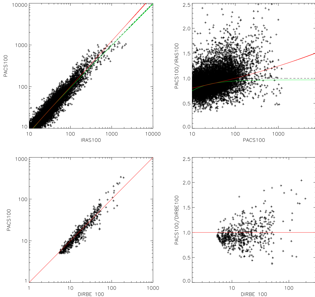
Fig. 9.— Pixel-to-pixel correlation between the convolved, resampled PACS 100 \mu\text{m} combined map of the LMC and the IRAS 100 \mu\text{m} image on the one hand (top) and the DIRBE 100 \mu\text{m} map on the other hand (bottom). Surface brightnesses are plotted in MJy/sr. In the top panel, the green line shows a bisector linear fit to the correlation, yielding a slope of 0.97. The red line shows an exponential fit, leading to (\text{PACS}/50 \text{ MJy/sr}) = 0.94 (\text{IRAS}/50 \text{ MJy/sr})^{1.09} . In the bottom panel, the red line indicates a 1:1 correlation.
