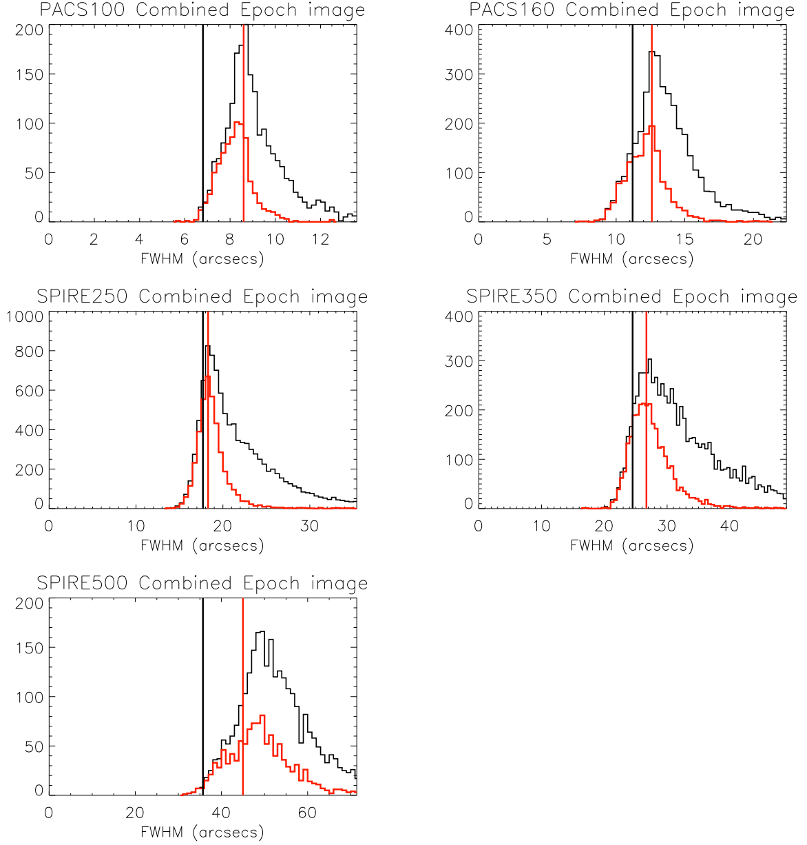
Fig. 20.— Plotted are histograms of the FWHM (average of the x and y directions) of HERITAGE catalog sources. The black histograms show all sources that could be fit with a Gaussian in both x and y directions. Sources with the lowest sky values (40% of total) are plotted in red. This shows that sources on higher background sky areas tend to produce higher FWHM values. This can be attributed to extended emission of the source, or to the more difficult task of separating the point source from the background emission. The black vertical line is the FWHM (2D average) of the initial Herschel -supplied PSFs, and the red vertical line is the FWHM of the broadened PSFs that were used to produce the HERITAGE catalogs. The SPIRE 500 \mu\text{m} PSF values suffer the most from background sky contamination.
