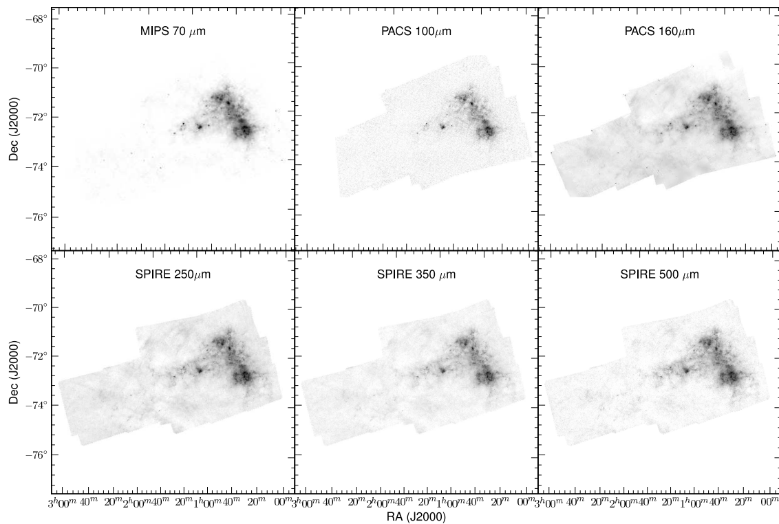
Fig. 15.— The HERITAGE data for the SMC with the Spitzer -SAGE-SMC MIPS 70 \mu\text{m} image (Gordon et al. 2011) for comparison. Together these data sets sample the spectral energy distribution of ISM dust emission. The grey scale displays are all in arcsinh with the following ranges: MIPS 70 \mu\text{m} , 0–100 MJy sr ^{-1} ; PACS 100 \mu\text{m} 3–250 MJy sr ^{-1} ; PACS 160 \mu\text{m} 5–200 MJy sr ^{-1} ; SPIRE 250 \mu\text{m} 0–100 MJy sr ^{-1} ; SPIRE 350 \mu\text{m} 0–80 MJy sr ^{-1} ; SPIRE 500 \mu\text{m} 0–30 MJy sr ^{-1} .
