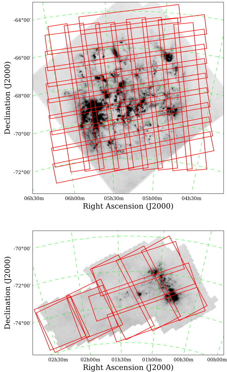
Fig. 1.— The HERITAGE SPIRE AOR mapping strategy for the LMC (top) and SMC (bottom) overlaid on the MIPS 160\ \mu\text{m} image from the SAGE-LMC Spitzer Legacy program (Meixner et al. 2006) and SAGE-SMC Spitzer Legacy program (Gordon et al. 2011). Each long red rectangle represents the footprint of one AOR (see Table 2 for details on sizes). The long scans of each epoch are sufficient to get off the main galaxy far-infrared emissions and sample a suitable background. The AORs for both epoch 1 and epoch 2 are shown. Because the epochs were separated in time by approximately 3 months, the AORs are orthogonal and the combination of both epoch footprints results in a basketweave appearance. This observing strategy improved the final photometry quality of the combined epoch maps.
