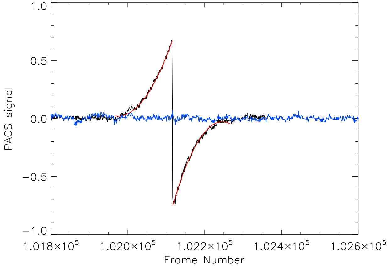
Fig. 7.— Manifestation of a long glitch in the PACS 100 \mu\text{m} timelines. The black line shows the uncorrected timeline, with the discontinuity at frame number \simeq 1.021 \times 10^5 caused by the glitch. The red line corresponds to a polynomial fit of order 2 to the 150 frames on each side of the discontinuity. The blue line shows the corrected timeline (glitch removed).
