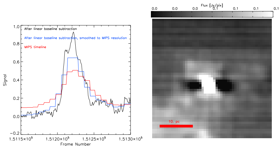
Fig. 3.— Baseline subtraction and point sources. Left: Example of point source morphology mismatch between the smoothed PACS and the MIPS 160 \mu\text{m} timelines. The black line shows the roughly baseline subtracted PACS timeline, corresponding to the timeline in the second panel in Figure 2. The red line shows the MIPS timeline, as in the third panel of Figure 2. The blue line shows the roughly baseline subtracted, smoothed PACS timeline, as panel 3 of Figure 2. Right: Effects in the projected maps of over-subtraction around bright/compact sources due to differences in the shapes of the MIPS and PACS timelines caused by the one-dimensionality of the convolution. This problem is solved by linearly interpolating the timeline inside such regions.
