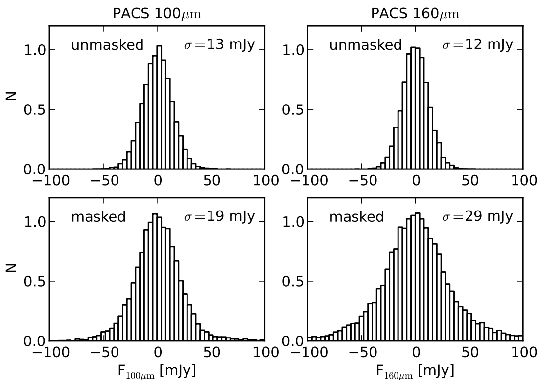
Fig. 22.— Histograms showing the distribution of the aperture photometry of 10,000 apertures on the LMC PACS residual minus sky image. The histograms are normalized to peak at N=1 . PACS 100 \mu\text{m} is shown to the left and PACS 160 \mu\text{m} to the right. The scatter of the flux (quantified with the standard deviation, \sigma ) is indicated in each panel for apertures in unmasked (top row) and masked (bottom row) regions.
