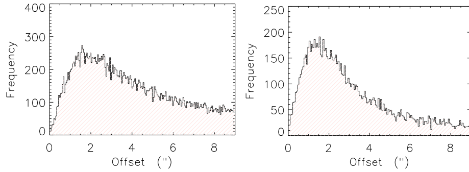
Fig. 12.— Left panel: The histogram of positional offsets between the SPIRE 250\ \mu\text{m} point source locations and their corresponding MIPS 24\ \mu\text{m} point source locations for the LMC. Frequency is the number of sources with a particular offset. Right panel: Similar positional histogram offsets but for the SMC.
