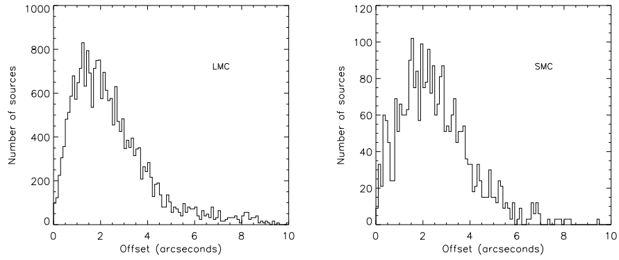
Fig. 6.— Left panel: The histogram of positional offsets between the PACS 160 \mu\text{m} point source locations and their corresponding MIPS 24 \mu\text{m} point source locations for the LMC. Right panel: Similar positional histogram offsets but for the SMC.
