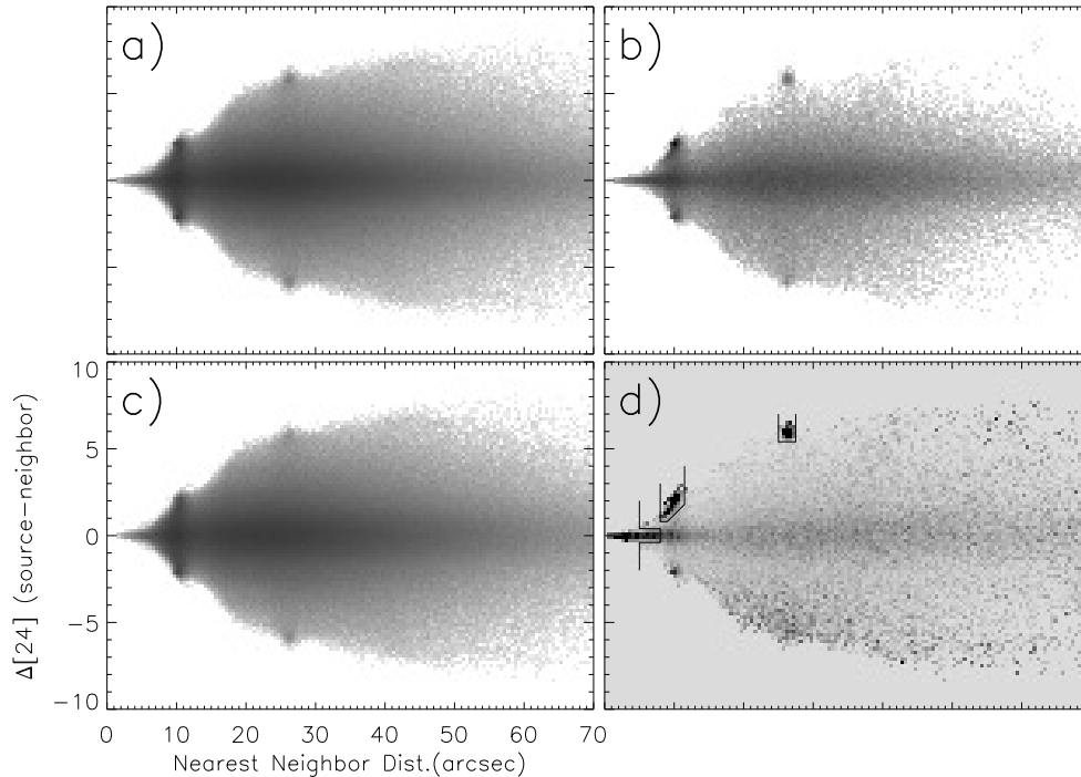
Fig. 4.— Density maps of the magnitude difference between each source and its nearest neighbor versus their separation distance in arcseconds. In panel a), we plot data for the entire archive. We split the set between those sources that lack or possess GLIMPSE counterparts in panels b) and c) respectively. Finally, panel d) shows a map of statistically significant ( >3\sigma in black) overdensities in panel b) relative to panel c); black lines mark our conditions for flagging a source as “confused” and therefore not included in the high quality catalog data product. The inverted grayscale is logarithmic in panels a), b), & c), with white for <1 source per bin. Black is >10^3 sources per bin in panel b) and >10^4 in a) & c). Panel d) is linear scaled from -0.5 to 3, white to black.
