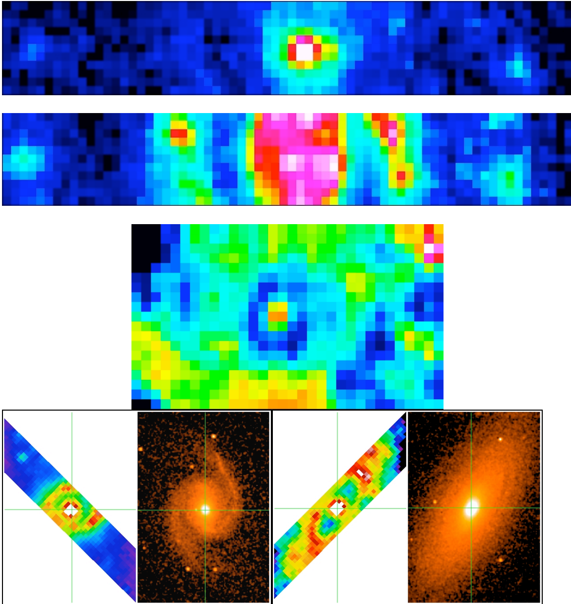
Figure 2. Top 3 panels are examples of DR5 products for NGC 5194. Top panel is the central portion of the continuum-subtracted [NeIII] emission. It is highly centrally concentrated compared to the continuum-subtracted [SiII] emission, shown in the second panel; it shows bright emission in the nucleus and the spiral arms. The third panel shows the integrated PAH emission at 8\mu\text{m} . The fourth and fifth panels show a side-by-side comparison of a 2MASS K-band image and a LL1 map for NGC 1566 and NGC 2841 respectively. The IRS maps have very good astrometry, typically within 1'' of the 2MASS coordinates, as indicated by the cross hairs in the last two panels.
